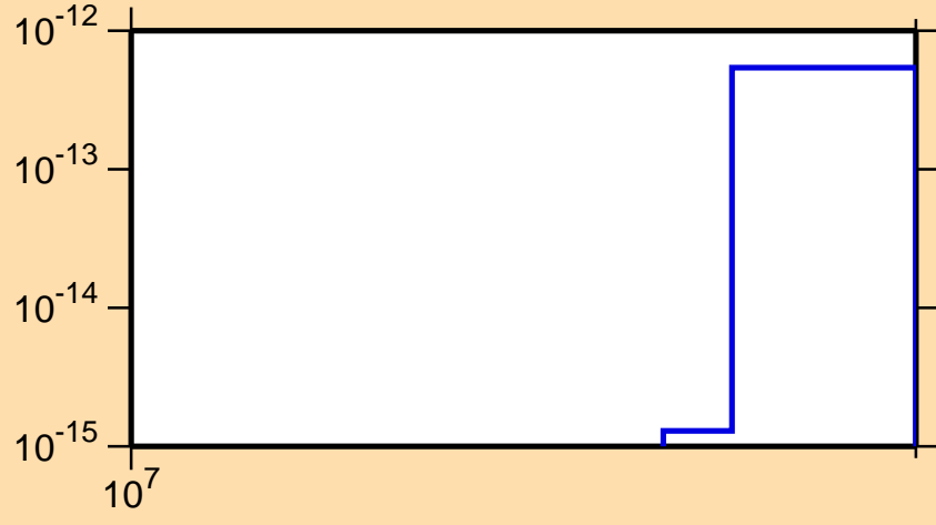
\sigma vs. E for ^{119}\text{In}(n,2n\alpha)
