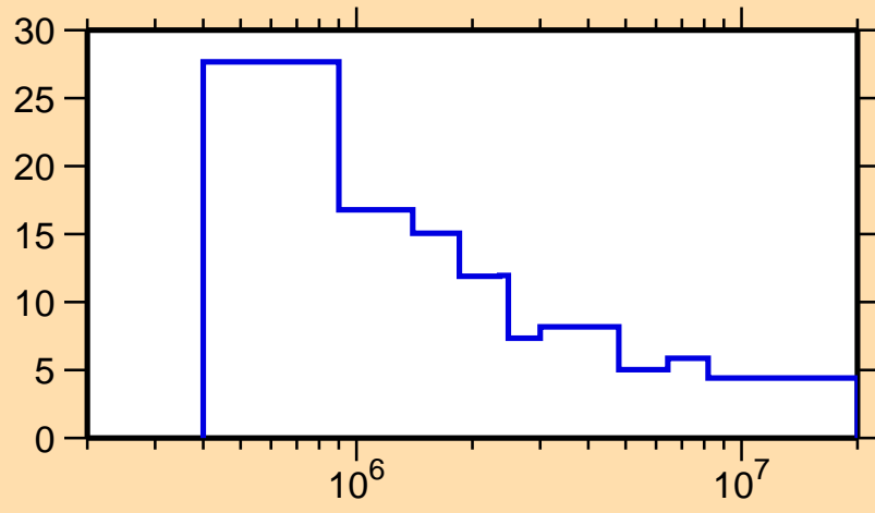
\Delta\sigma/\sigma vs. E for ^{120}\text{In}(n, n_{\text{nonel}})
