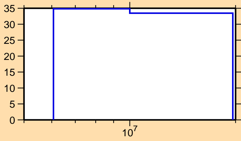
\Delta\sigma/\sigma vs. E for ^{121}\text{In}(n,n_1)
