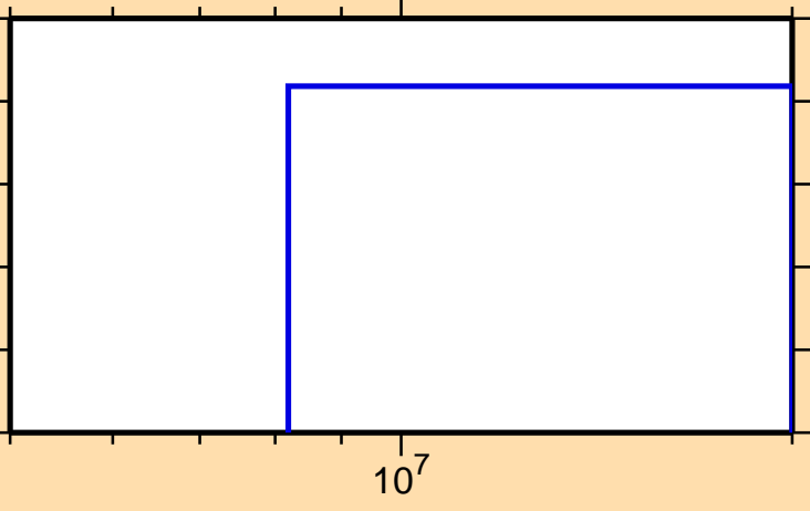
\sigma vs. E for ^{121}\text{In}(n,n\alpha)
