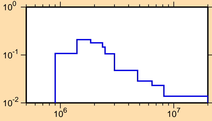
\sigma vs. E for ^{121}\text{In}(n,n_4)
