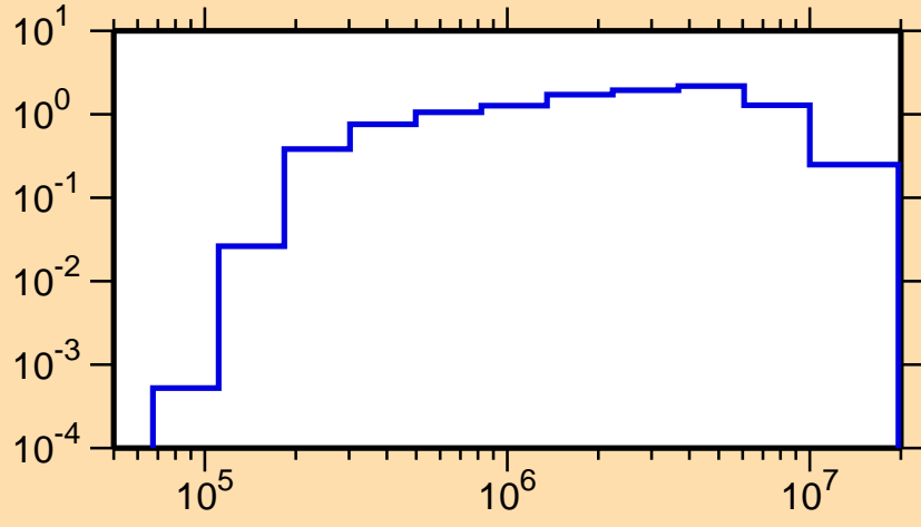
\sigma vs. E for ^{122}\text{In}(n,\text{inel.})
