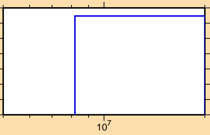
\sigma vs. E for ^{122}\text{In}(n,np)
