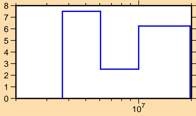
\Delta\sigma/\sigma vs. E for ^{122}\text{In}(n,\text{tot.})
