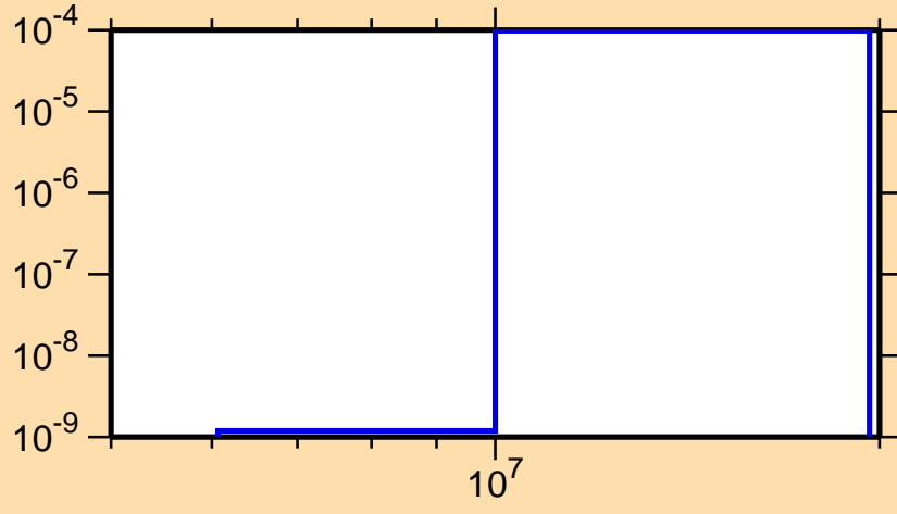
\sigma vs. E for ^{122}\text{In}(n,\alpha)
