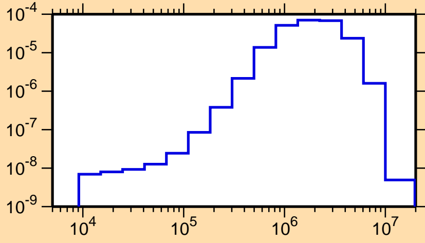
\sigma vs. E for ^{122}\text{In}(n,n_1)
