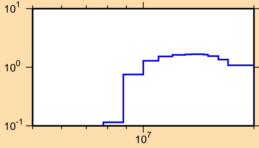
\sigma vs. E for ^{123}\text{In}(n,2n)
