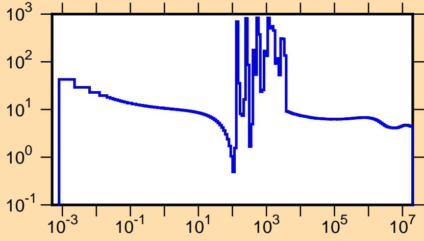
\sigma vs. E for ^{123}\text{In}(n,\text{tot.})
