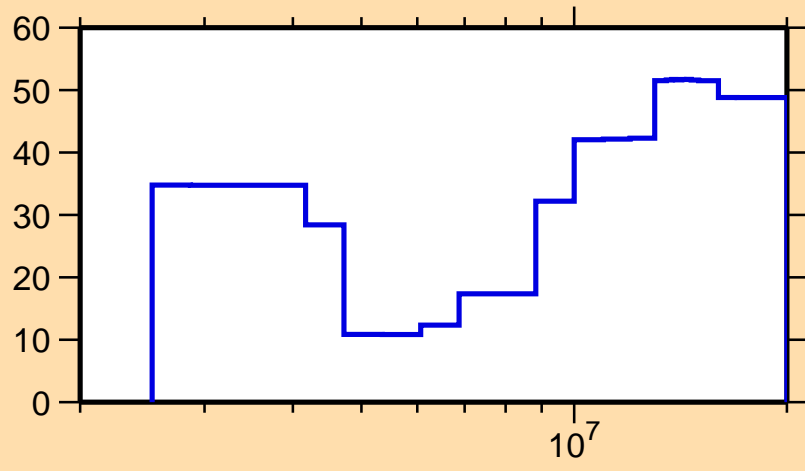
\Delta\sigma/\sigma vs. E for ^{123}\text{In}(n,n\text{cont.})
