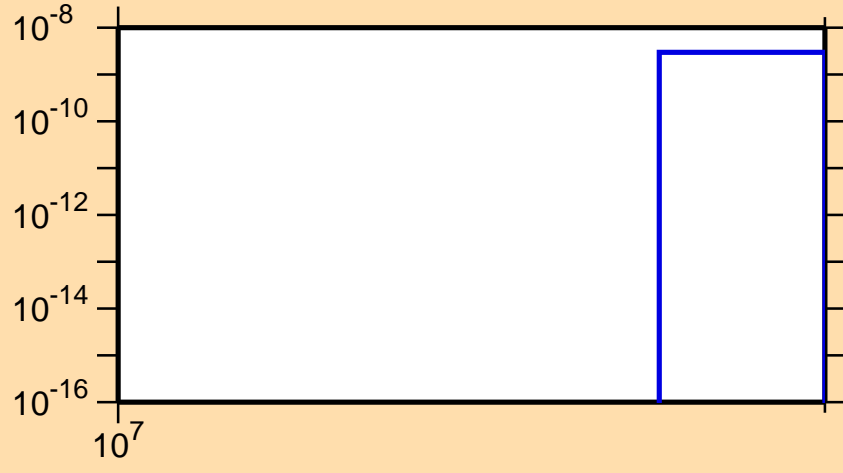
\sigma vs. E for ^{123}\text{In}(n,nd)
