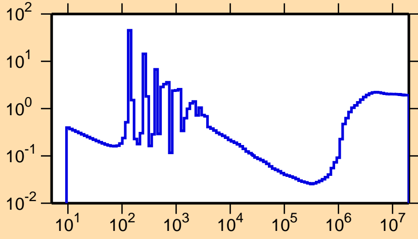
\sigma vs. E for ^{123}\text{In}(n,\text{nonel.})
