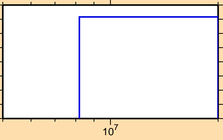
\sigma vs. E for ^{123}\text{In}(n,n\alpha)
