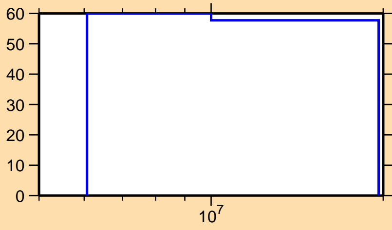
\Delta\sigma/\sigma vs. E for ^{124}\text{In}(n,n_1)
