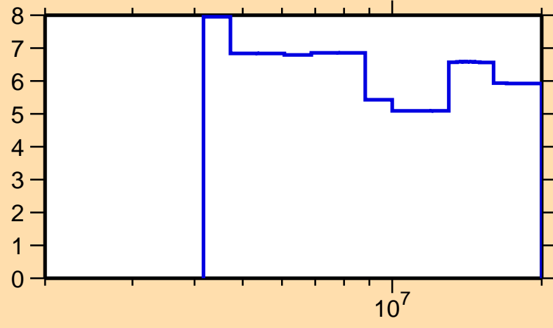
\Delta\sigma/\sigma vs. E for ^{124}\text{In}(n,\text{nonel.})
