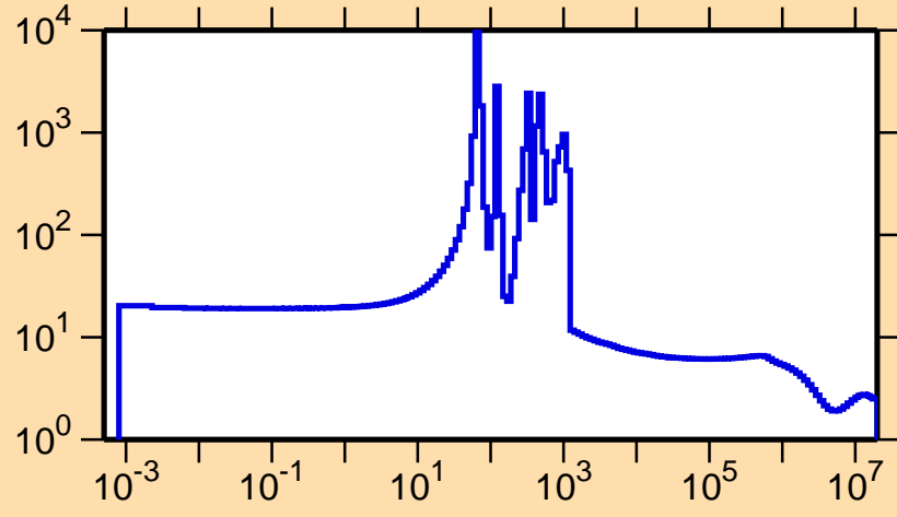
\sigma vs. E for ^{124}\text{In}(n,\text{el.})
