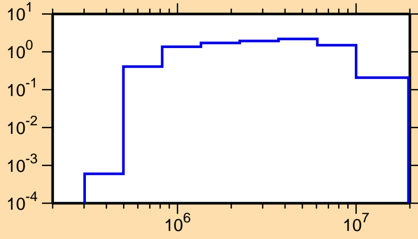
\sigma vs. E for ^{124}\text{In}(n,\text{inel.})
