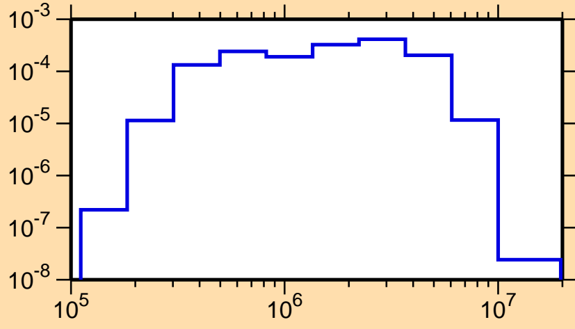
\sigma vs. E for ^{124}\text{In}(n,n_4)
