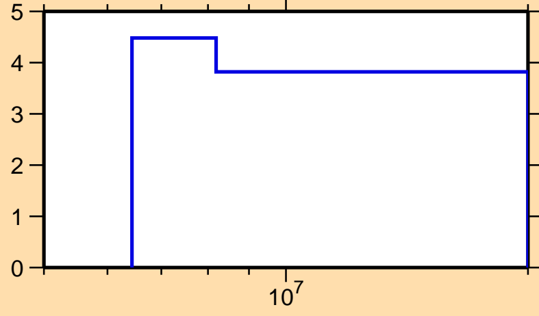
\Delta\sigma/\sigma vs. E for ^{124}\text{In}(n,\text{tot.})
