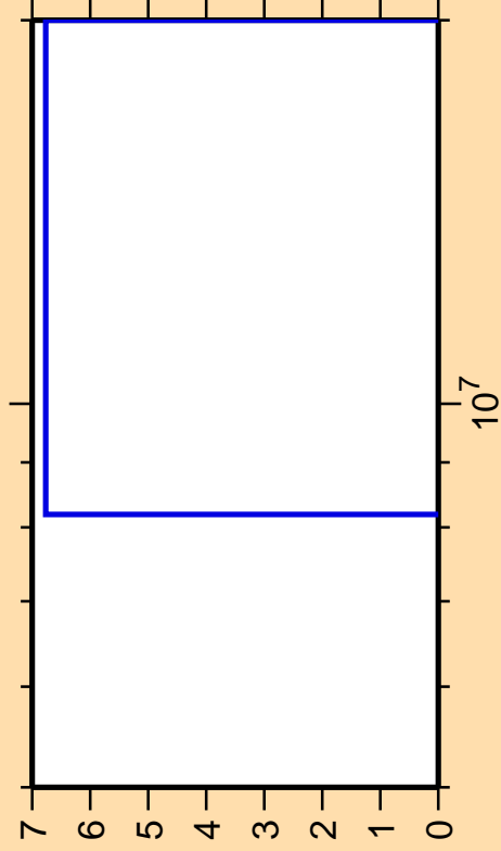
\Delta\sigma/\sigma vs. E for ^{124}\text{In}(n,2np)
