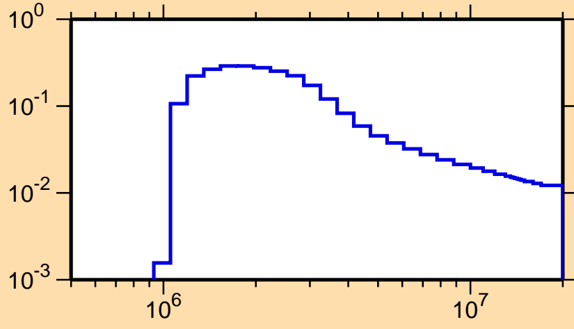
\sigma vs. E for ^{125}\text{In}(n,n_3)
