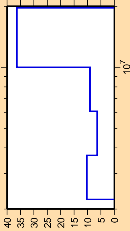
\Delta\sigma/\sigma vs. E for ^{125}\text{In}(n,n\text{cont.})
