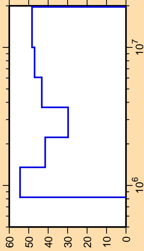
\Delta\sigma/\sigma vs. E for ^{125}\text{In}(n,n_3)
