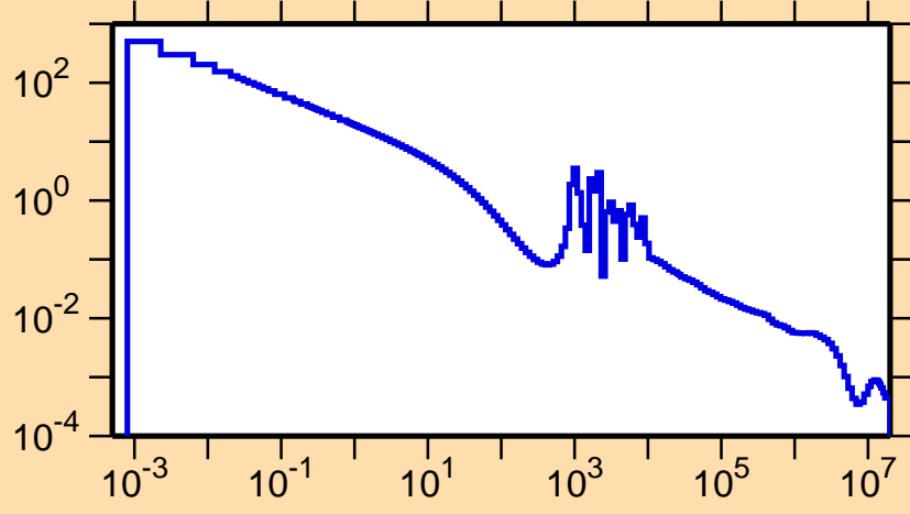
\sigma vs. E for ^{125}\text{In}(n,\gamma)
