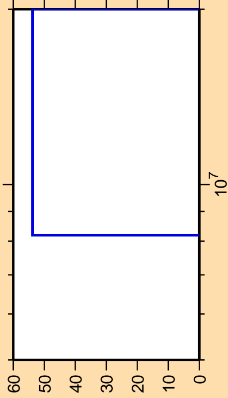
\Delta\sigma/\sigma vs. E for ^{125}\text{In}(n,nd)
