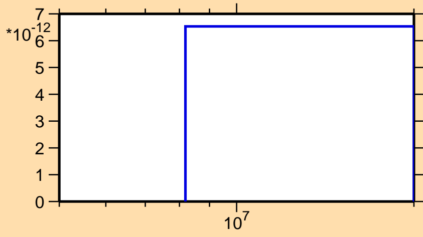
\sigma vs. E for ^{125}\text{In}(n,nd)
