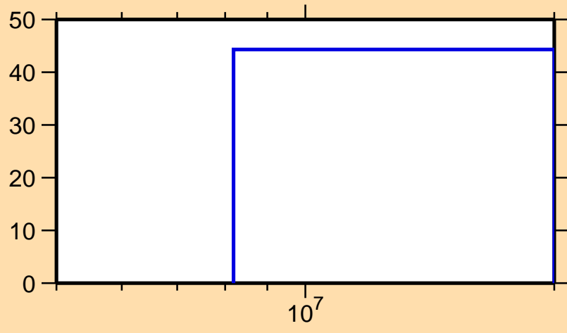
\Delta\sigma/\sigma vs. E for ^{126}\text{In}(n,n_1)
