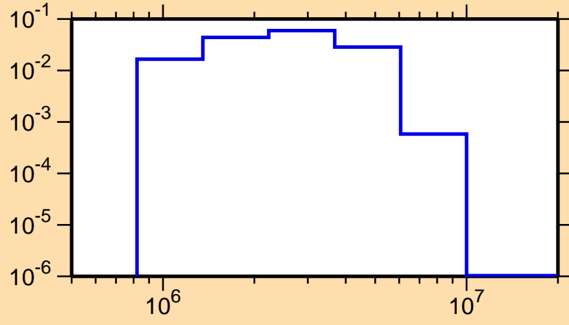
\sigma vs. E for ^{127}\text{In}(n,n_2)
