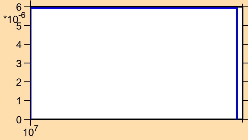
\sigma vs. E for ^{127}\text{In}(n,d)
