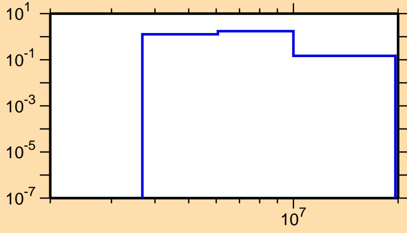
\sigma vs. E for ^{127}\text{In}(n,n\text{cont.})
