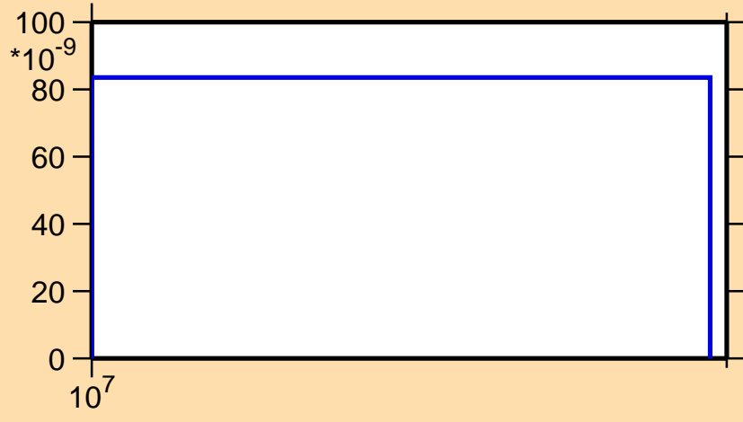
\sigma vs. E for ^{127}\text{In}(n,t)
