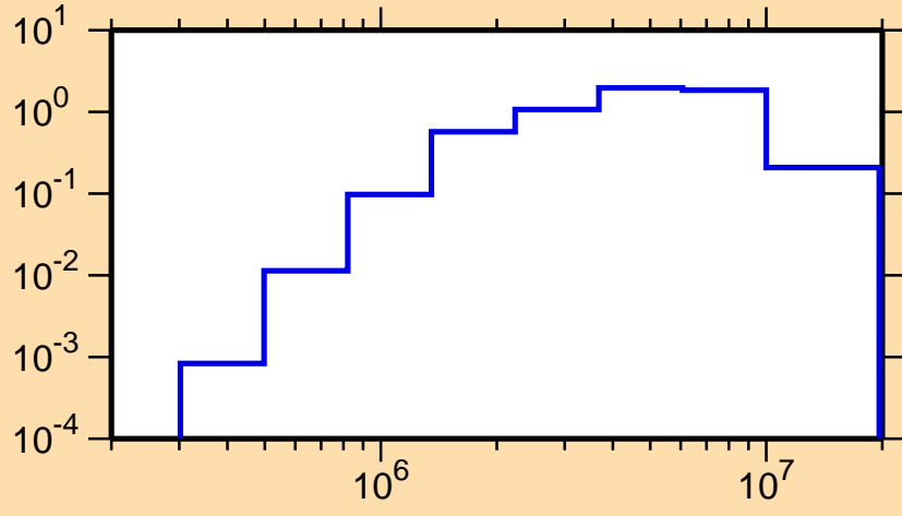
\sigma vs. E for ^{127}\text{In}(n,\text{inel.})
