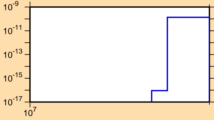
\sigma vs. E for ^{127}\text{In}(n,\text{nd})
