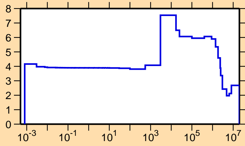
\sigma vs. E for ^{127}\text{In}(n,\text{el.})
