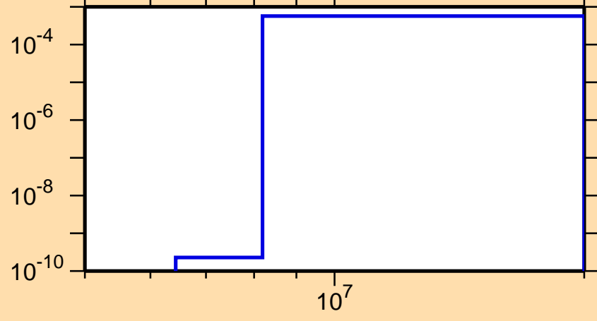
\sigma vs. E for ^{127}\text{In}(n,p)
