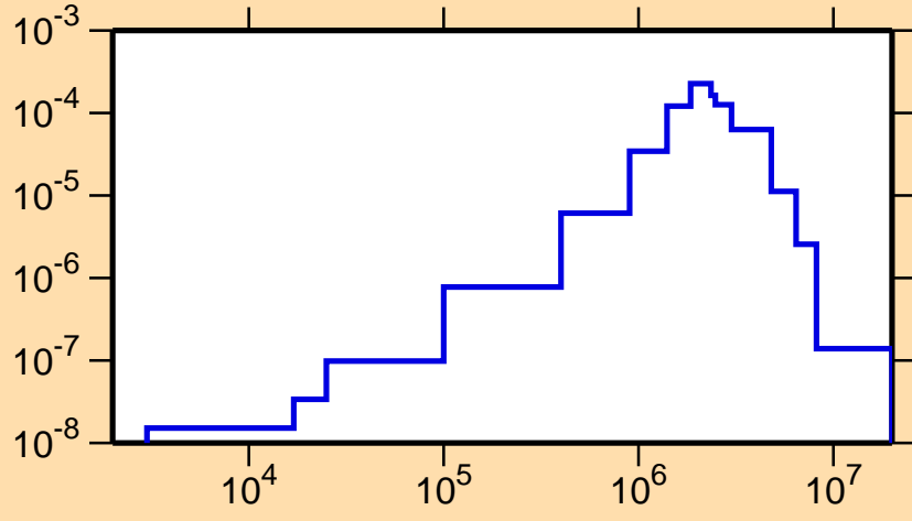
\sigma vs. E for ^{127}\text{In}(n,n_3)
