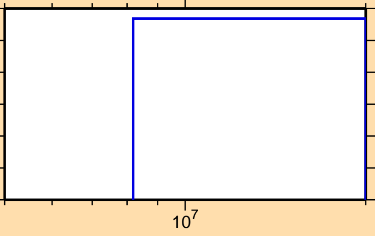
\sigma vs. E for ^{127}\text{In}(n,\alpha)
