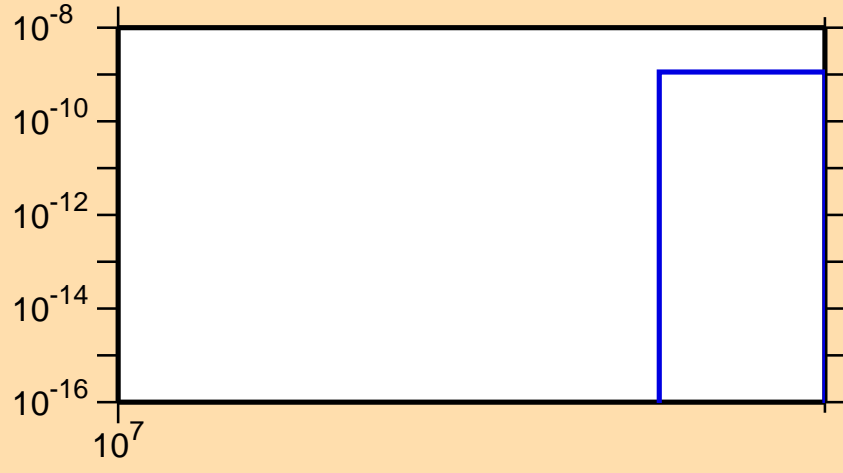
\sigma vs. E for ^{129}\text{In}(n,nt)
