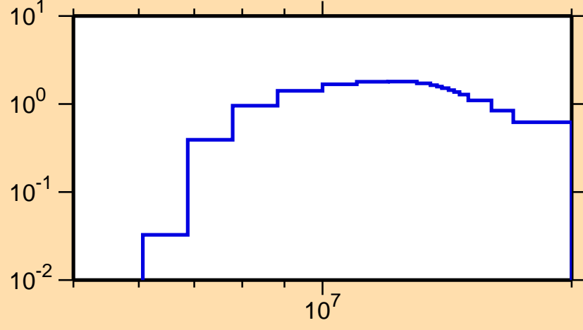
\sigma vs. E for ^{129}\text{In}(n,2n)
