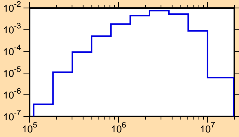
\sigma vs. E for ^{129}\text{In}(n,n_4)
