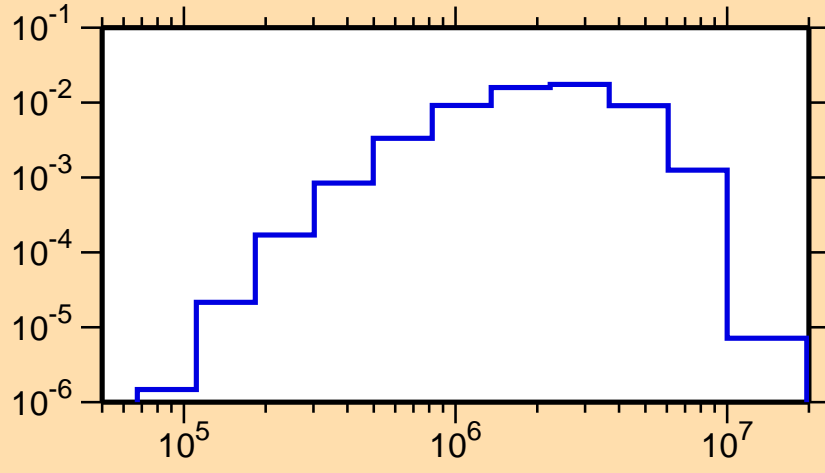
\sigma vs. E for ^{129}\text{In}(n,n_3)
