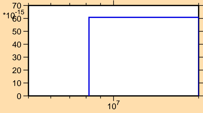
\sigma vs. E for ^{129}\text{In}(n,nd)
