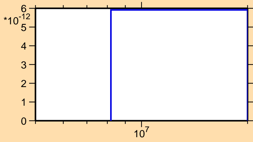
\sigma vs. E for ^{129}\text{In}(n,n\alpha)
