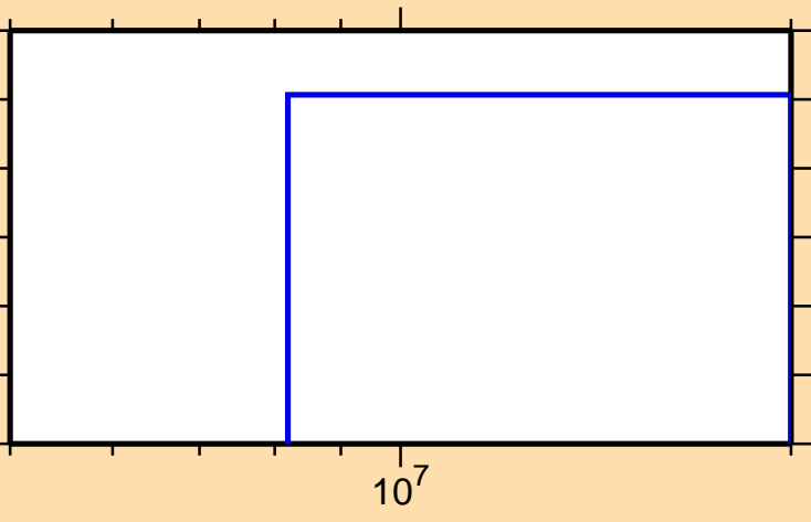
\sigma vs. E for ^{129}\text{In}(n,\alpha)
