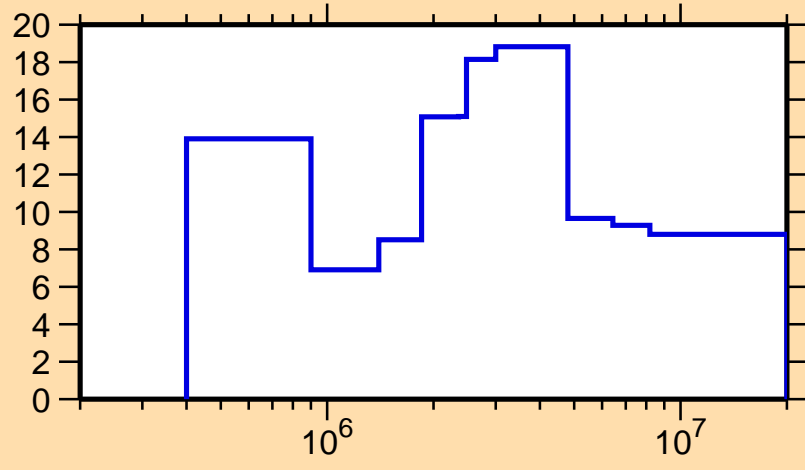
\Delta\sigma/\sigma vs. E for ^{129}\text{In}(n, el.)
