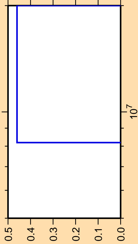
\Delta\sigma/\sigma vs. E for ^{129}\text{In}(n,nd)
