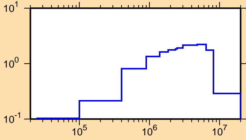
\sigma vs. E for ^{129}\text{In}(n,\text{inel.})
