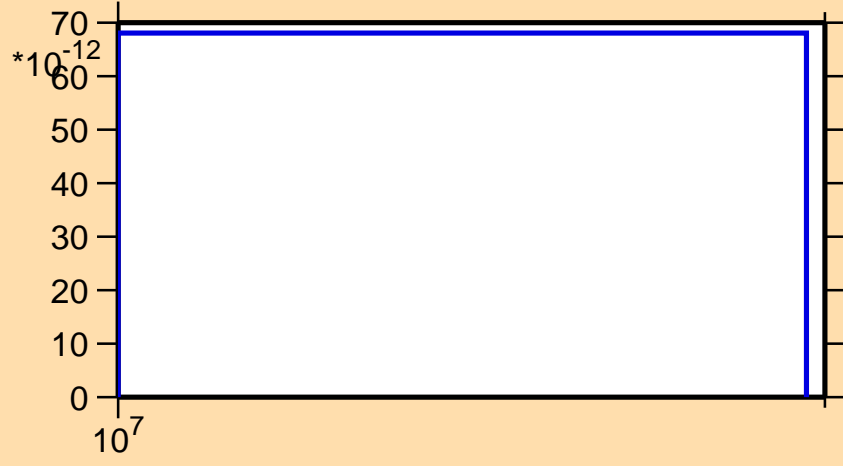
\sigma vs. E for ^{171}\text{Ir} (mt 34)
