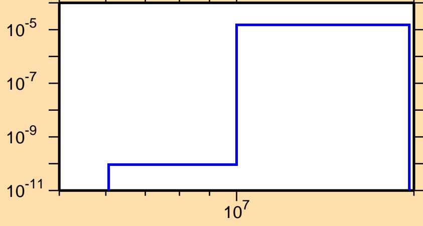
\sigma vs. E for ^{171}\text{Ir}(n,\text{pd})
