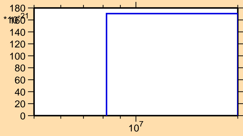
\sigma vs. E for ^{171}\text{Ir}(\text{mt } 42)
