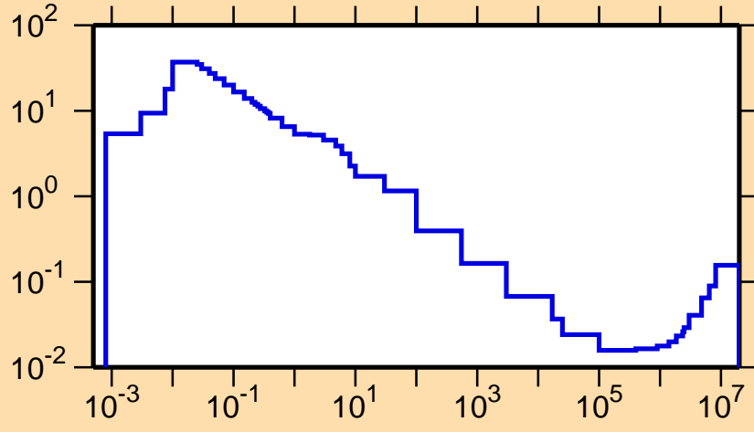
\sigma vs. E for ^{171}\text{Ir}(n,\alpha)
