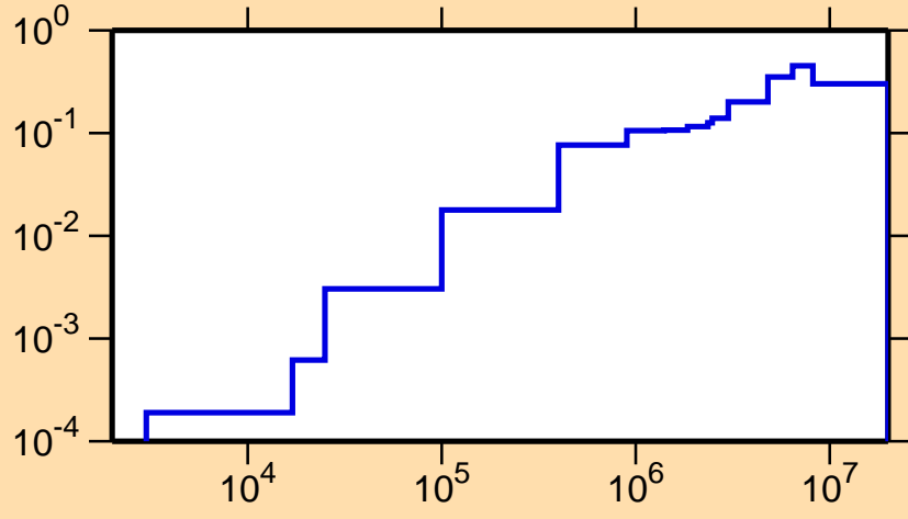
\sigma vs. E for ^{171}\text{Ir}(n,\text{inel.})
