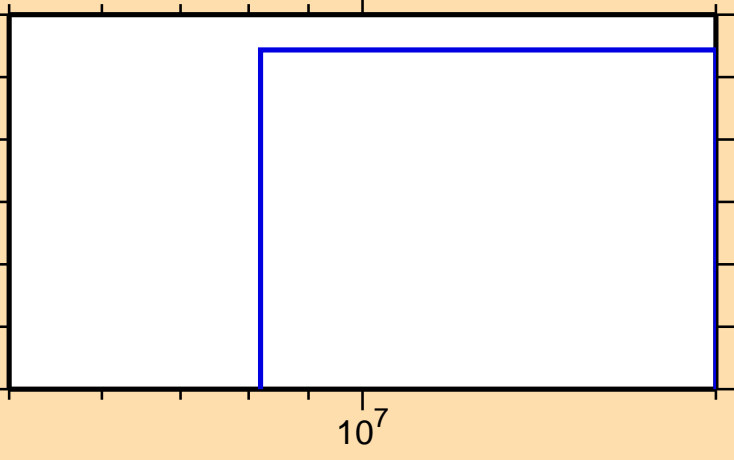
\sigma vs. E for ^{171}\text{Ir}(n,2n)
