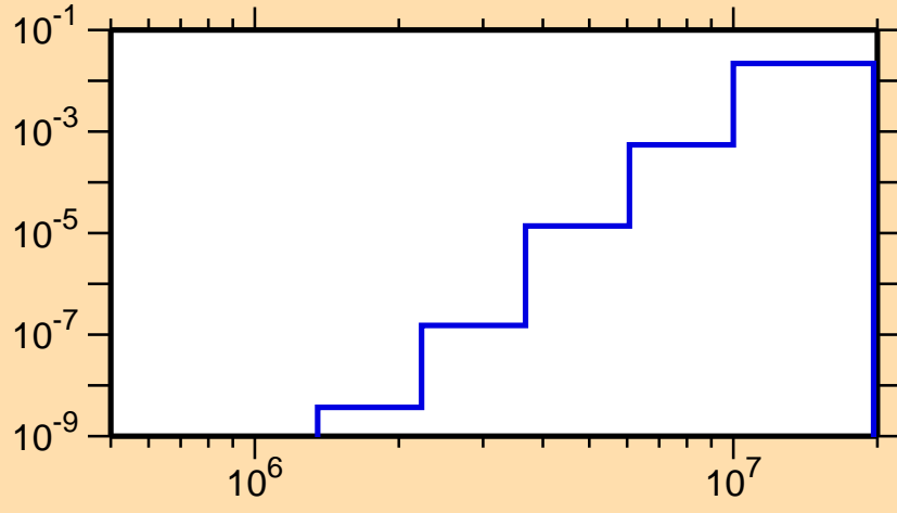
\sigma vs. E for ^{172}\text{Ir}(n,n\alpha)
