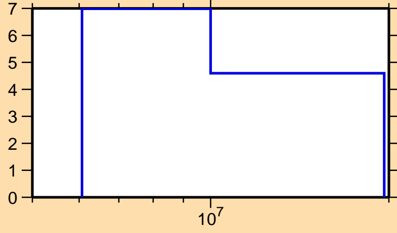
\Delta\sigma/\sigma vs. E for ^{172}\text{Ir}(n,\text{tot.})
