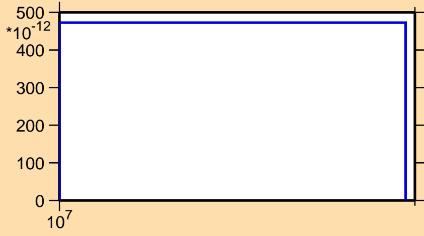
\sigma vs. E for ^{172}\text{Ir} (mt 34)
