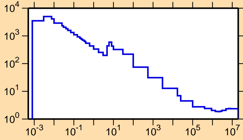
\sigma vs. E for ^{172}\text{Ir}(n,\text{nonel.})
