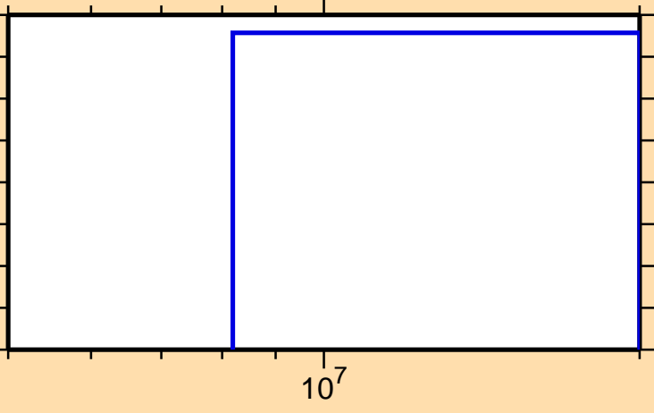
\sigma vs. E for ^{172}\text{Ir}(n,2n)
