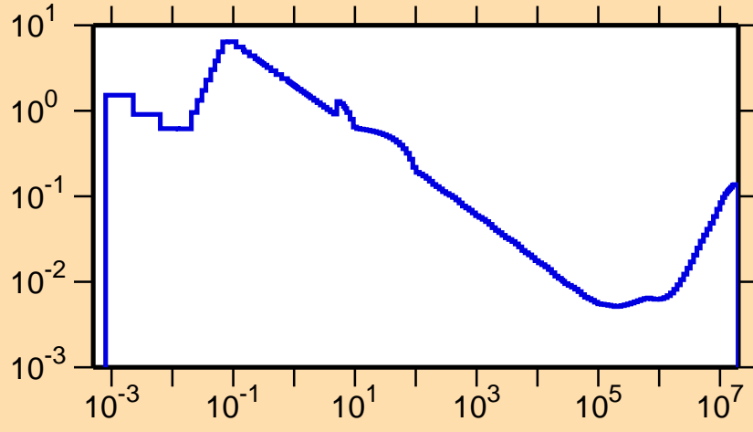
\sigma vs. E for ^{173}\text{Ir}(n,\alpha)
