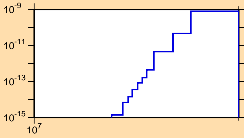
\sigma vs. E for ^{173}\text{Ir}(\text{mt } 34)
