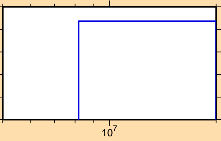
\sigma vs. E for ^{173}\text{Ir}(n,2np)
