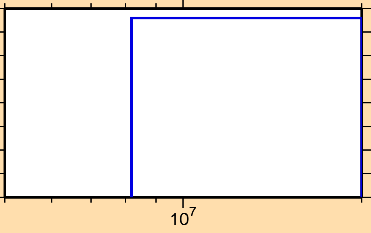
\sigma vs. E for ^{173}\text{Ir}(n,\text{nd})
