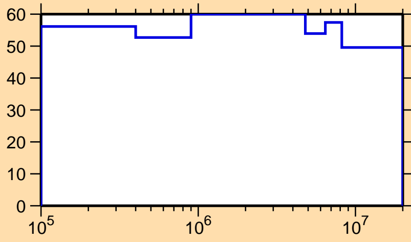
\Delta\sigma/\sigma vs. E for ^{173}\text{Ir}(n,n_1)
