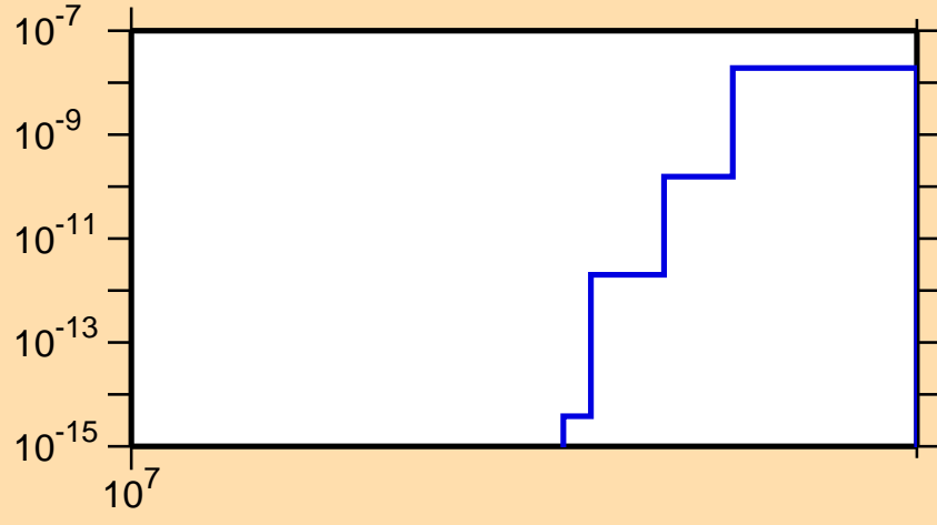
\sigma vs. E for ^{173}\text{Ir}(n,nt)
