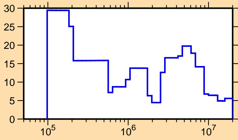
\Delta\sigma/\sigma vs. E for ^{173}\text{Ir}(n, el.)
