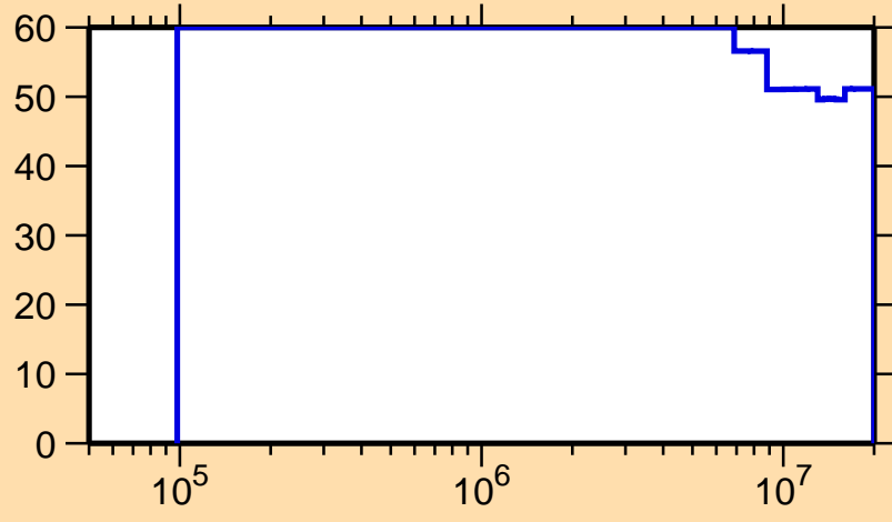
\Delta\sigma/\sigma vs. E for ^{173}\text{Ir}(n,n\text{cont.})
