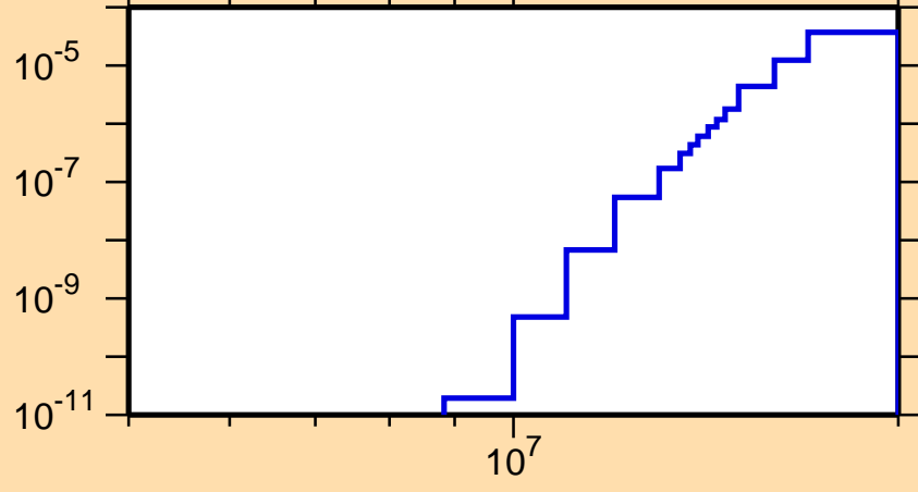
\sigma vs. E for ^{173}\text{Ir}(n,\text{pd})
