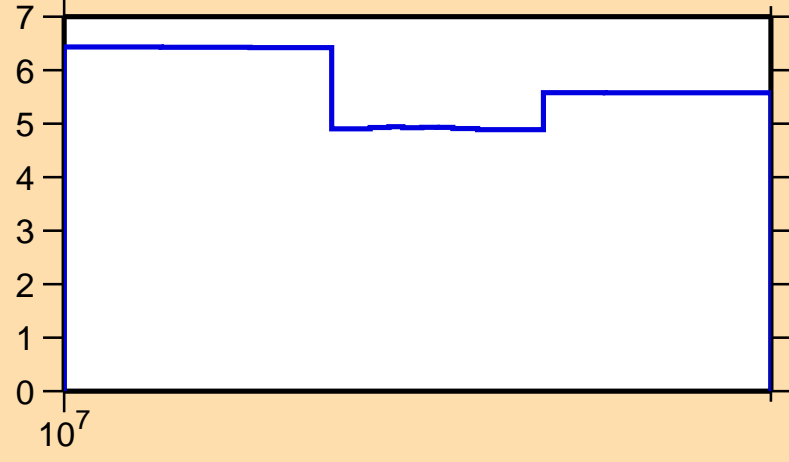
\Delta\sigma/\sigma vs. E for ^{173}\text{Ir}(n,\text{el.})
