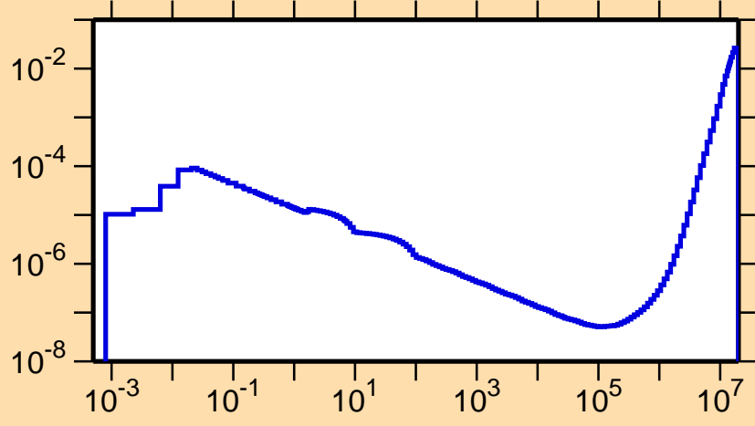
\sigma vs. E for ^{173}\text{Ir}(n,p\alpha)
