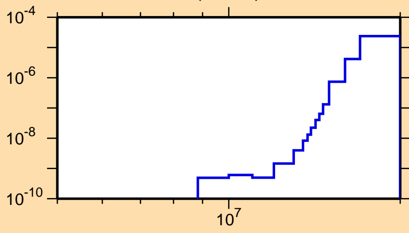
\sigma vs. E for ^{173}\text{Ir}(n,2n\alpha)
