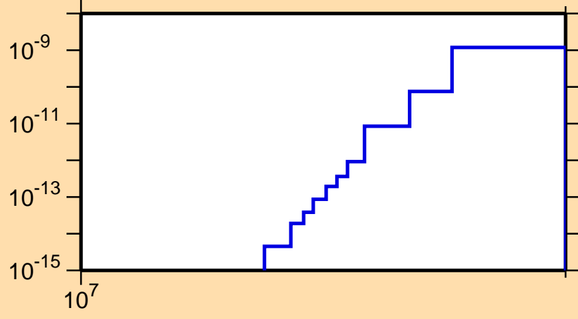
\sigma vs. E for ^{173}\text{Ir}(\text{mt } 34)
