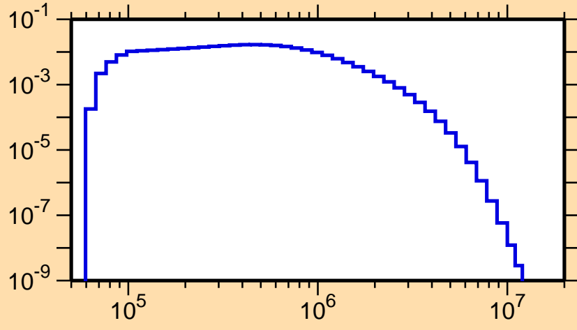
\sigma vs. E for ^{173}\text{Ir}(n,n_3)
