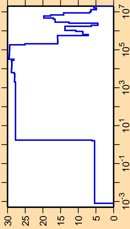
\Delta\sigma/\sigma vs. E for ^{173}\text{Ir}(n,\text{el.})
