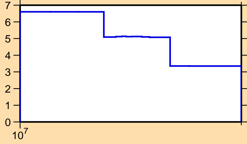
\Delta\sigma/\sigma vs. E for ^{173}\text{Ir}(n,\text{tot.})
