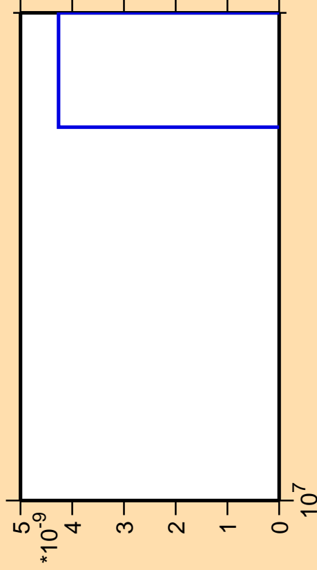
\Delta\sigma/\sigma vs. E for ^{173}\text{Ir} (mt 42)
