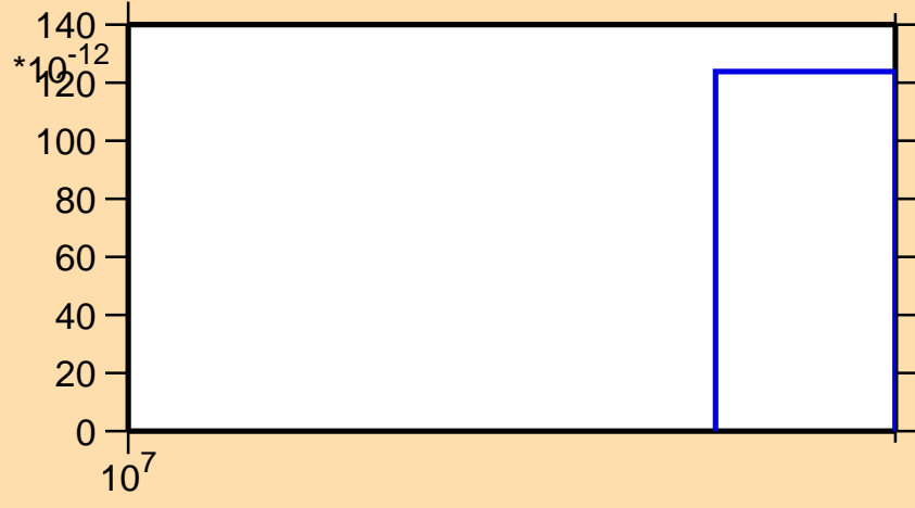
\sigma vs. E for ^{173}\text{Ir}(n,3n)
