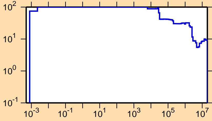
\Delta\sigma/\sigma vs. E for ^{173}\text{Ir}(n,\text{nonel.})
