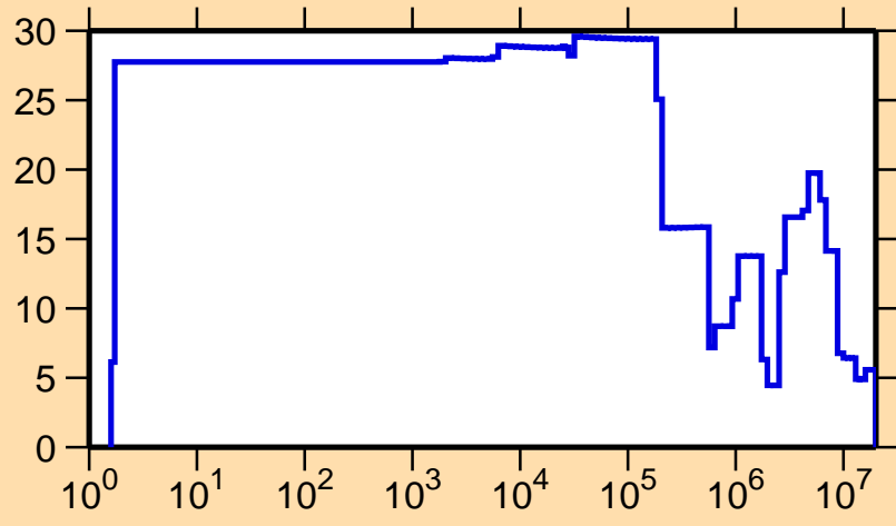
\Delta\sigma/\sigma vs. E for ^{173}\text{Ir}(n,\text{el.})
