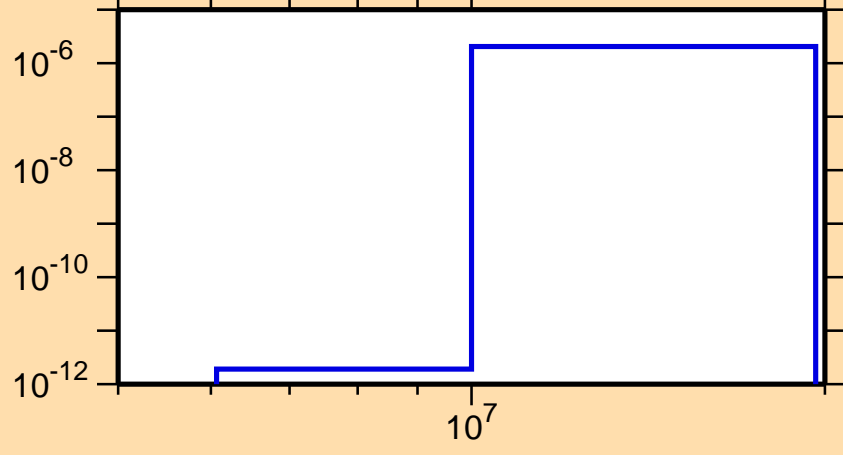
\sigma vs. E for ^{173}\text{Ir}(n,pd)
