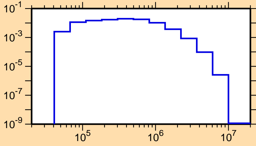
\sigma vs. E for ^{173}\text{Ir}(n,n_2)
