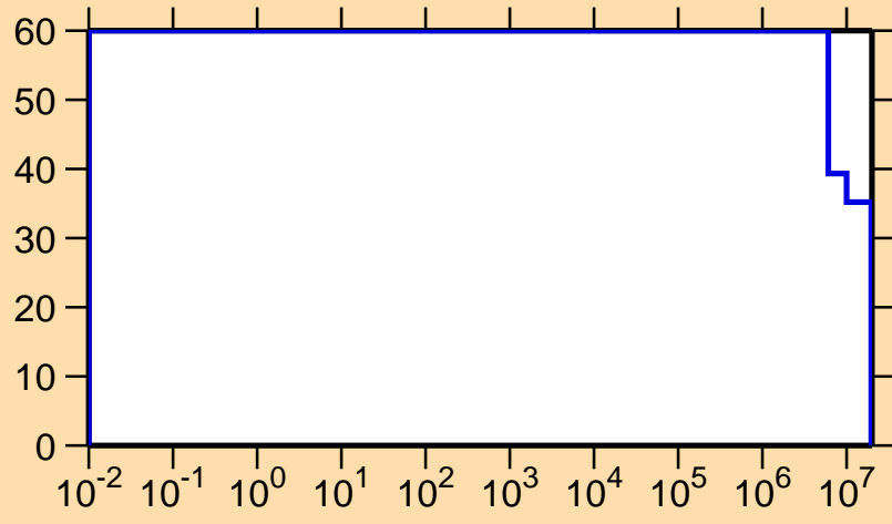
\Delta\sigma/\sigma vs. E for ^{173}\text{Ir}(n,p)
