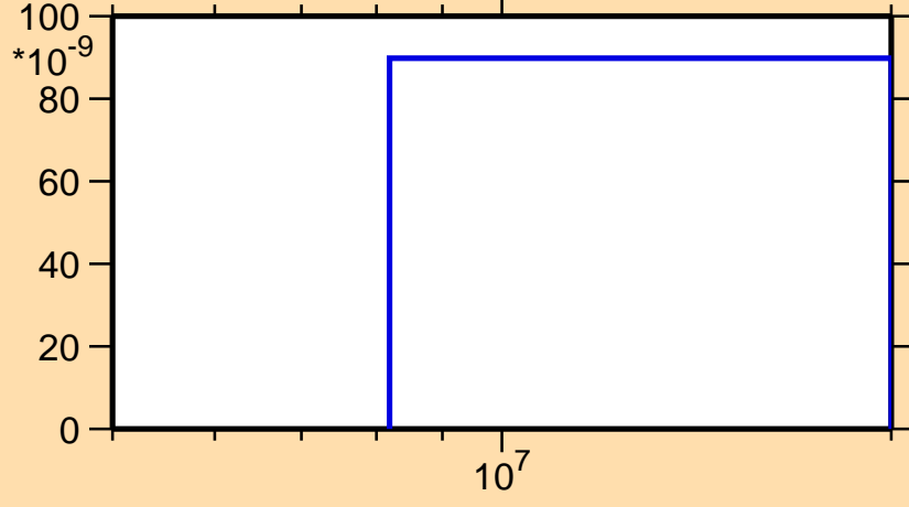
\sigma vs. E for ^{173}\text{Ir}(n,\text{nd})
