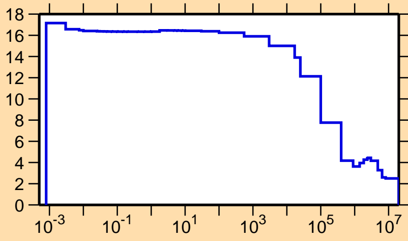
\sigma vs. E for ^{173}\text{Ir}(n,\text{el.})
