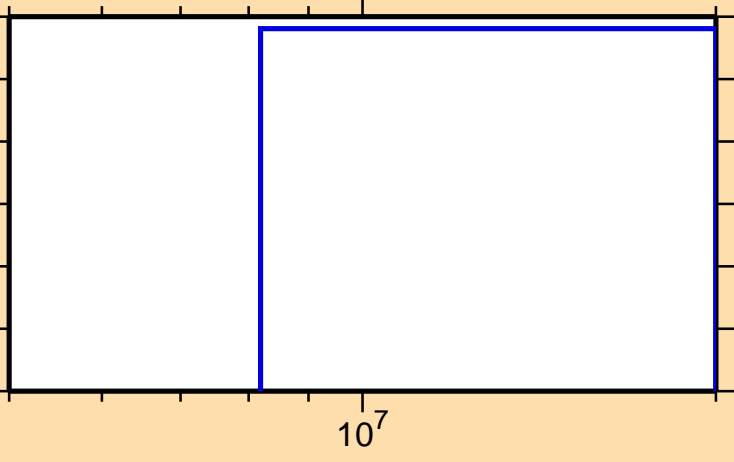
\sigma vs. E for ^{173}\text{Ir}(n,2np)
