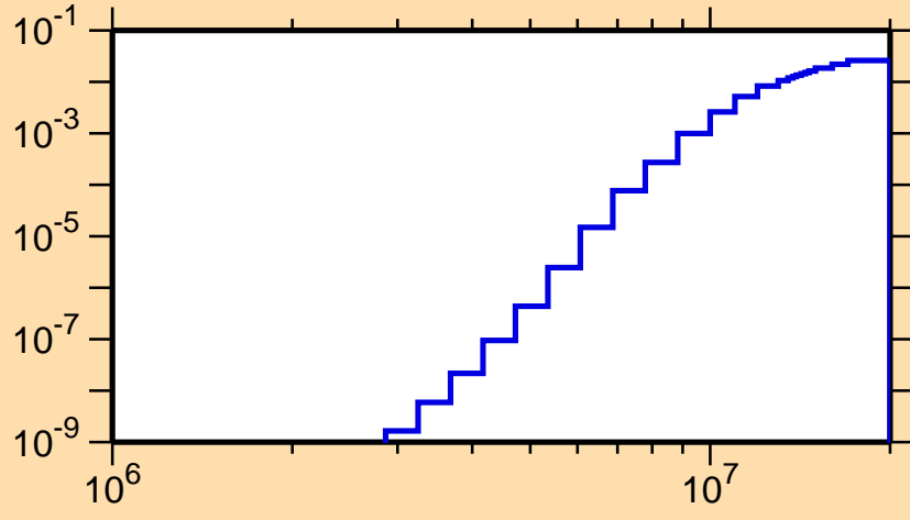
\sigma vs. E for ^{174}\text{Ir}(n,d)
