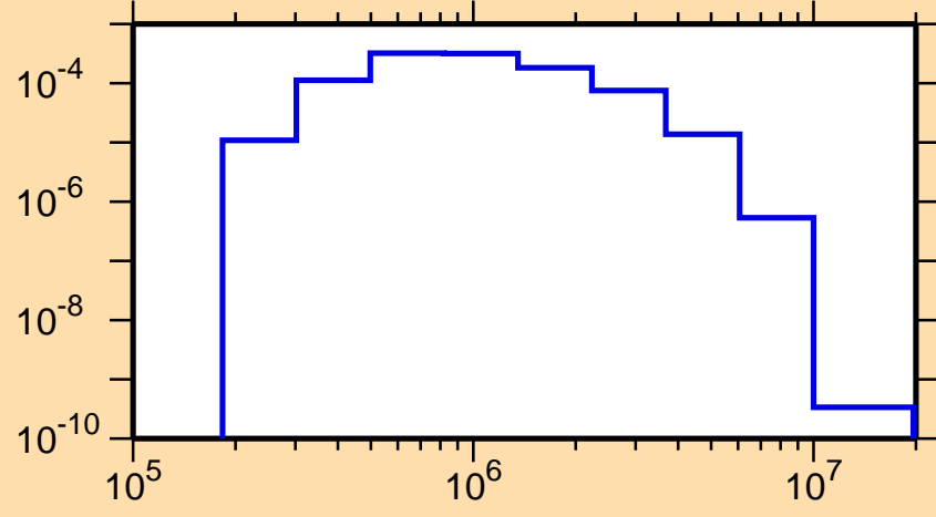
\sigma vs. E for ^{174}\text{Ir}(n,n_1)
