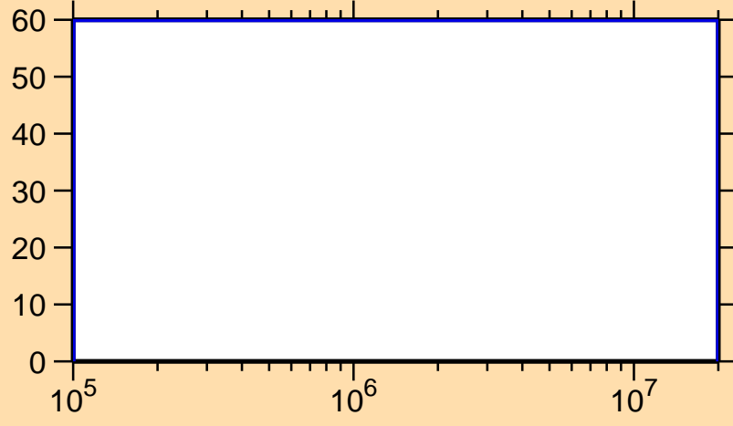
\Delta\sigma/\sigma vs. E for ^{174}\text{Ir}(n,n_1)
