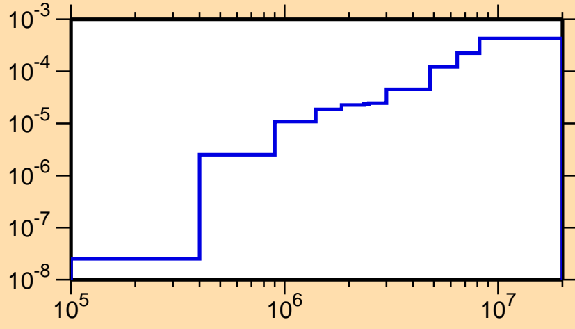
\sigma vs. E for ^{174}\text{Ir}(n,n_2)
