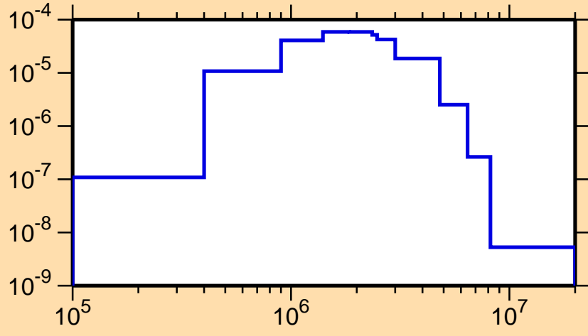
\sigma vs. E for ^{174}\text{Ir}(n,n_3)
