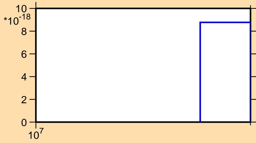
\sigma vs. E for ^{174}\text{Ir} (mt 42)
