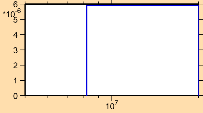
\sigma vs. E for ^{174}\text{Ir}(n,2n\alpha)
