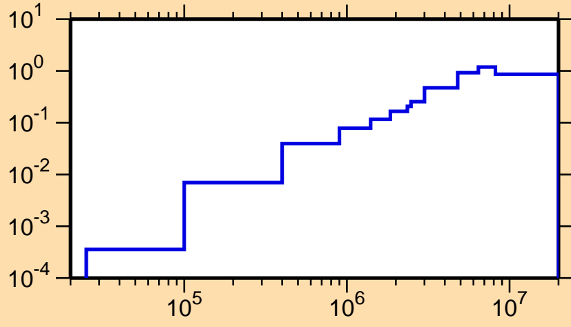
\sigma vs. E for ^{174}\text{Ir}(n,\text{inel.})
