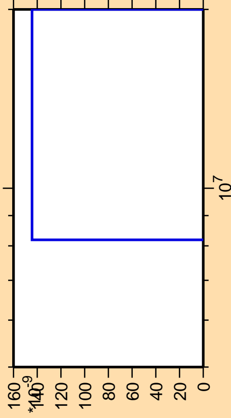
\Delta\sigma/\sigma vs. E for ^{174}\text{Ir}(\text{mt } 42)
