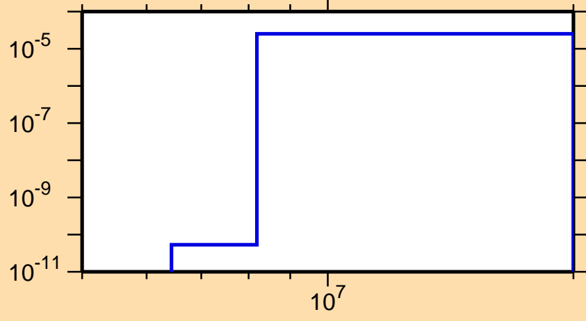
\sigma vs. E for ^{174}\text{Ir}(\text{mt } 45)
