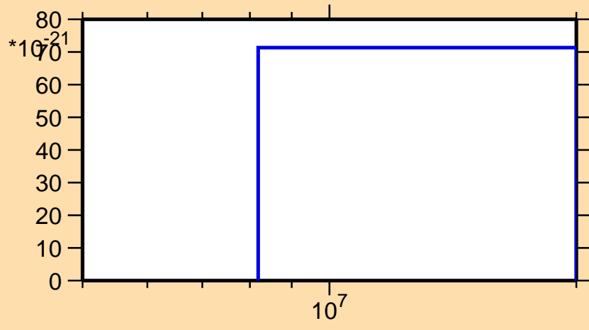
\sigma vs. E for ^{174}\text{Ir}(\text{mt } 42)
