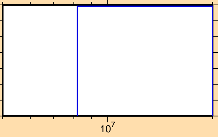
\sigma vs. E for ^{174}\text{Ir}(n,\text{pd})
