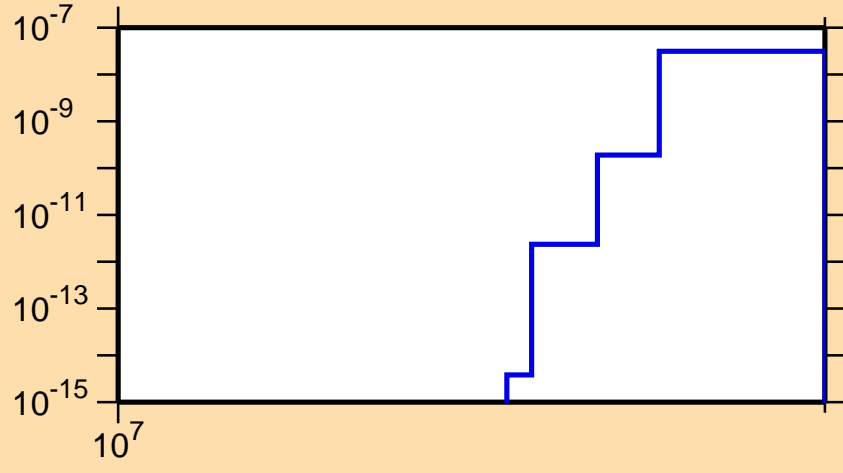
\sigma vs. E for ^{175}\text{Ir}(n,nt)
