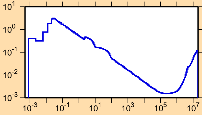
\sigma vs. E for ^{175}\text{Ir}(n,\alpha)
