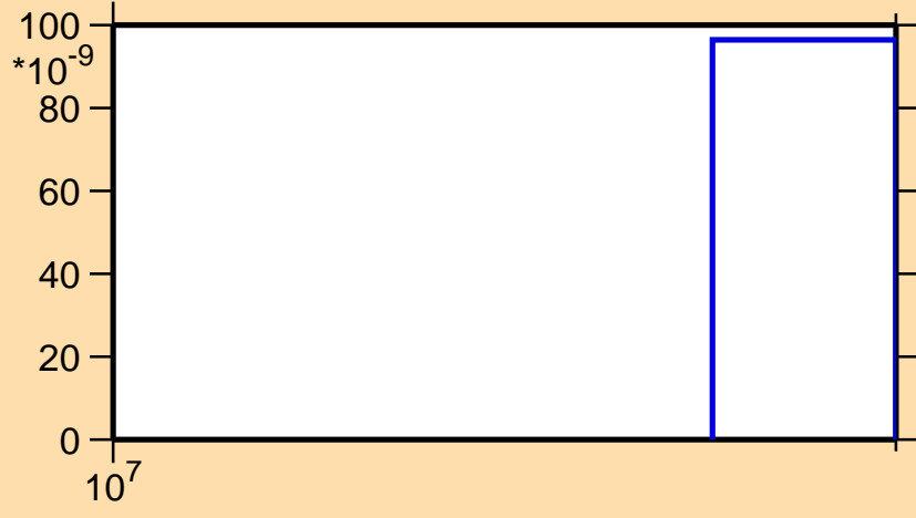
\sigma vs. E for ^{175}\text{Ir}(n,3n)
