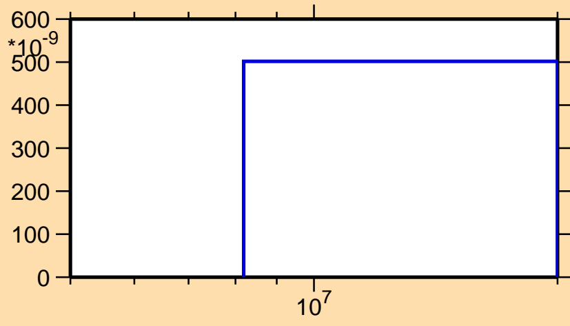
\sigma vs. E for ^{175}\text{Ir}(n,2n\alpha)
