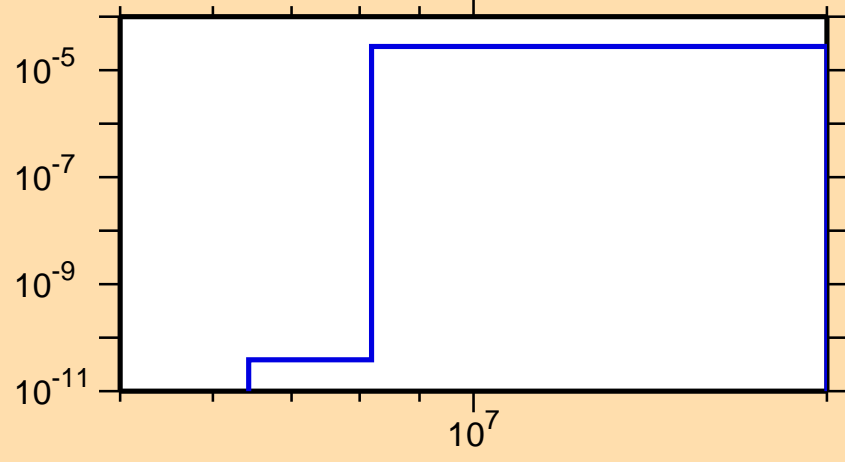
\sigma vs. E for ^{175}\text{Ir}(\text{mt } 45)
