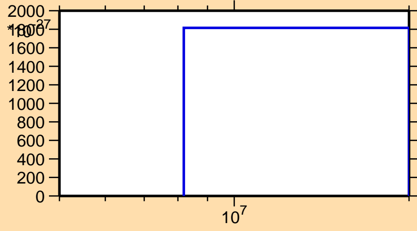
\sigma vs. E for ^{175}\text{Ir}(\text{mt } 42)
