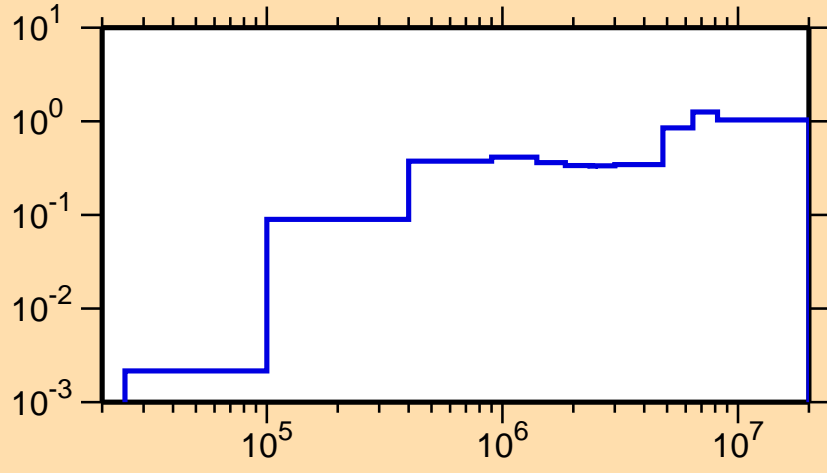
\sigma vs. E for ^{175}\text{Ir}(n,\text{inel.})
