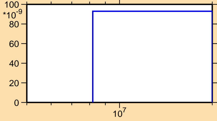
\sigma vs. E for ^{175}\text{Ir}(n,\text{nd})
