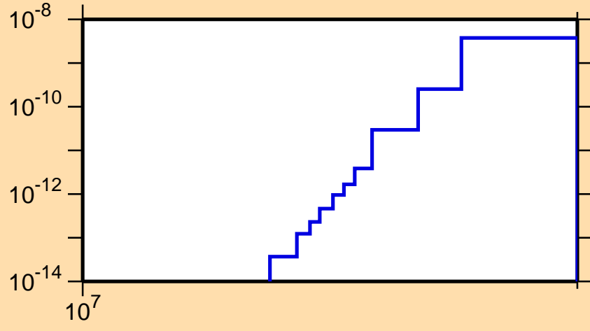
\sigma vs. E for ^{176}\text{Ir}(\text{mt } 34)
