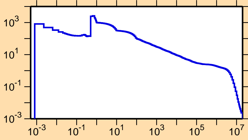
\sigma vs. E for ^{176}\text{Ir}(n,\gamma)
