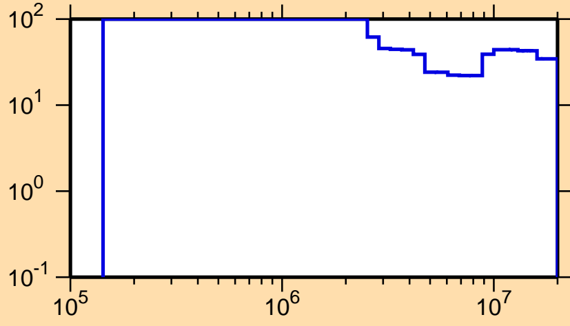
\Delta\sigma/\sigma vs. E for ^{176}\text{Ir}(n,n\text{cont.})
