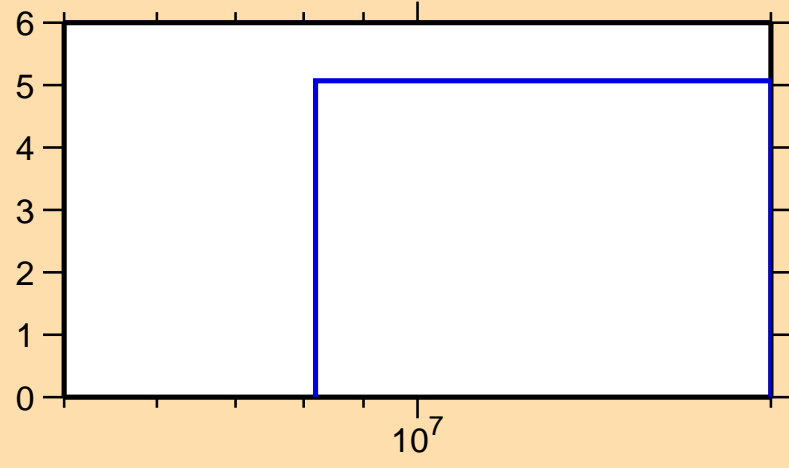
\Delta\sigma/\sigma vs. E for ^{176}\text{Ir}(n,\text{tot.})
