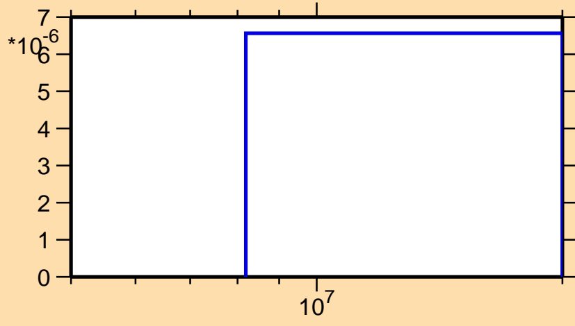
\sigma vs. E for ^{176}\text{Ir}(n,2n\alpha)
