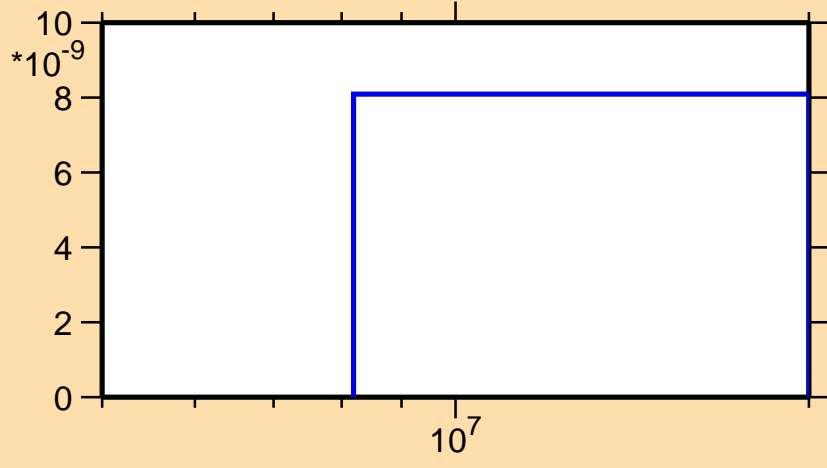
\sigma vs. E for ^{176}\text{Ir}(\text{mt117})
