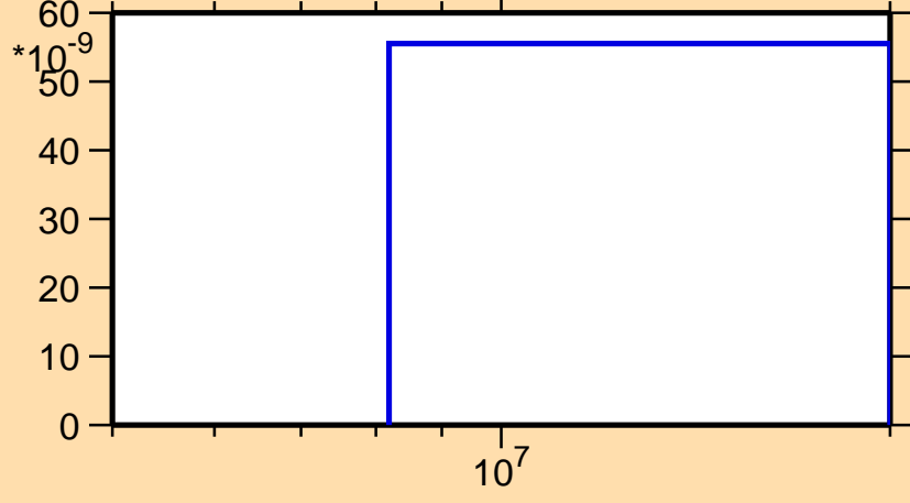
\sigma vs. E for ^{176}\text{Ir}(n,\text{pd})
