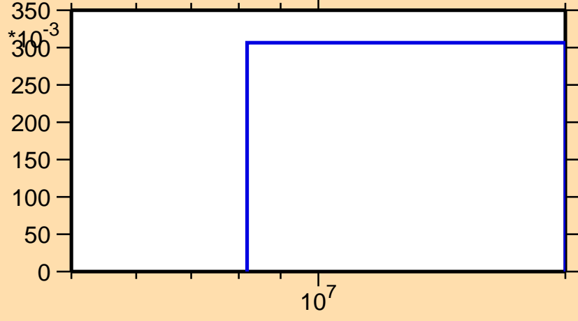
\sigma vs. E for ^{176}\text{Ir}(n,2n)
