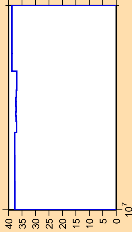
\Delta\sigma/\sigma vs. E for ^{177}\text{Ir}(n,n_1)
