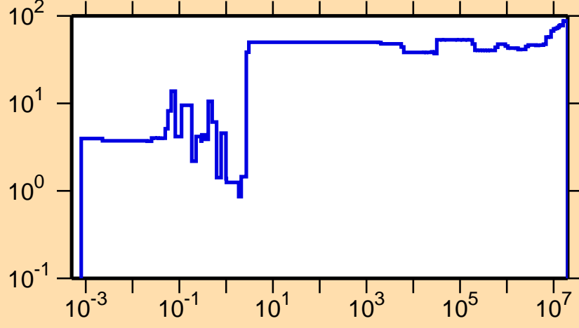
\Delta\sigma/\sigma vs. E for ^{177}\text{Ir}(n,\gamma)
