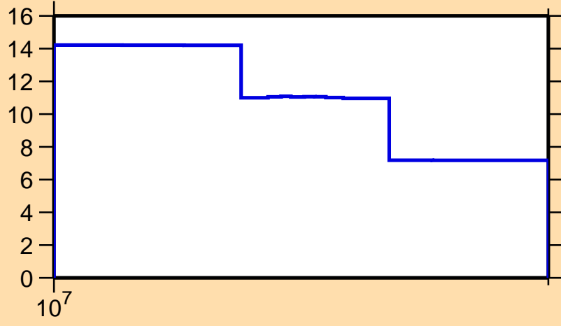
\Delta\sigma/\sigma vs. E for ^{177}\text{Ir}(n,\text{el.})
