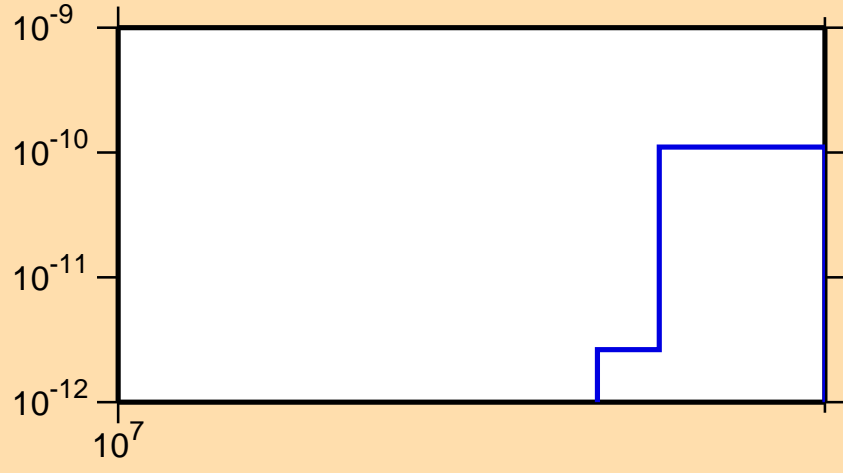
\sigma vs. E for ^{177}\text{Ir} (mt 34)
