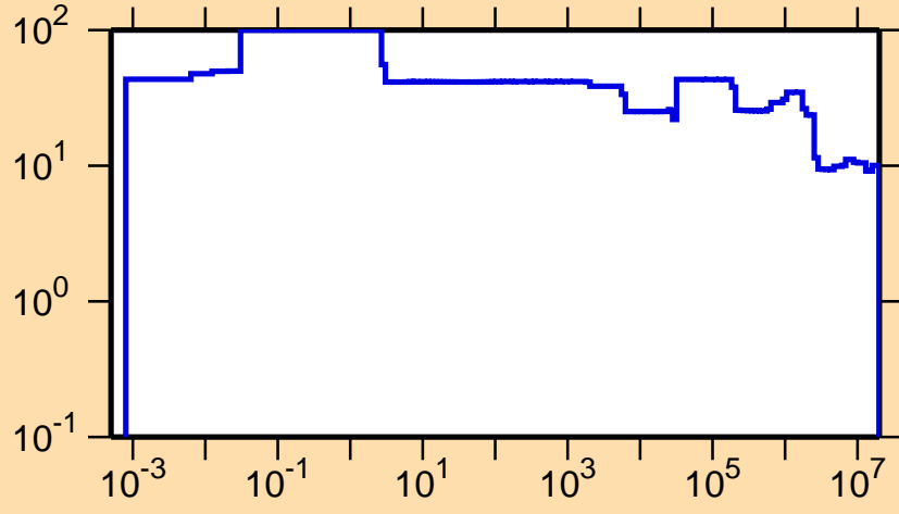
\Delta\sigma/\sigma vs. E for ^{177}\text{Ir}(n,\text{nonel.})
