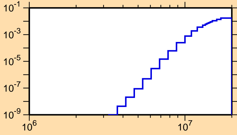
\sigma vs. E for ^{177}\text{Ir}(n,d)
