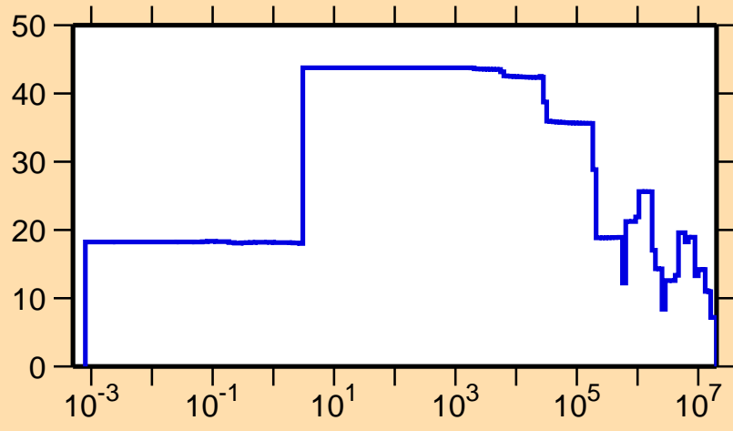
\Delta\sigma/\sigma vs. E for ^{177}\text{Ir}(n,\text{el.})
