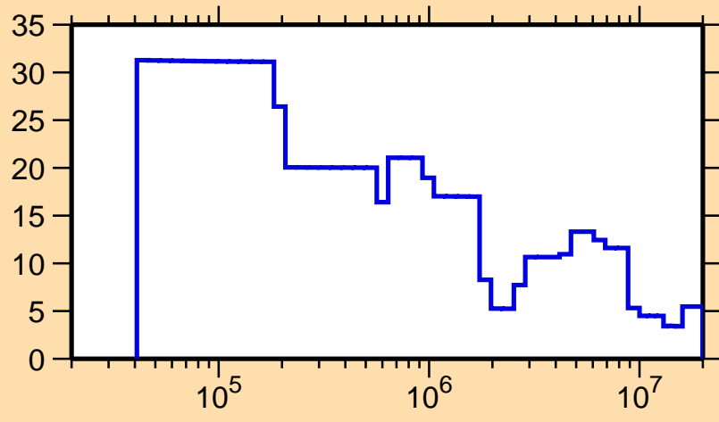
\Delta\sigma/\sigma vs. E for ^{177}\text{Ir}(n,\text{tot.})
