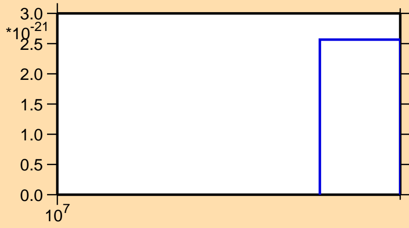
\sigma vs. E for ^{177}\text{Ir} (mt 42)
