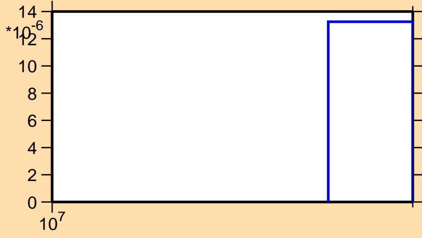
\sigma vs. E for ^{177}\text{Ir}(n,3n)
