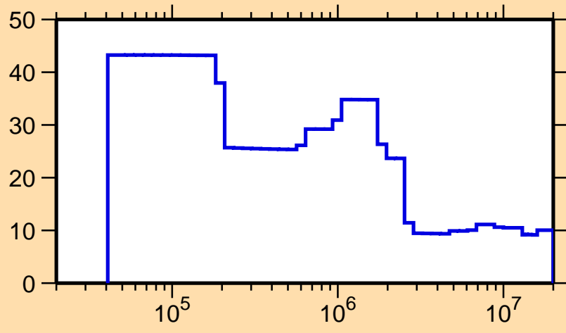
\Delta\sigma/\sigma vs. E for ^{177}\text{Ir}(n,\text{nonel.})
