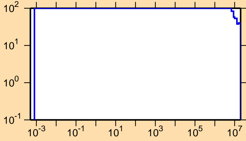
\Delta\sigma/\sigma vs. E for ^{177}\text{Ir}(n,p)
