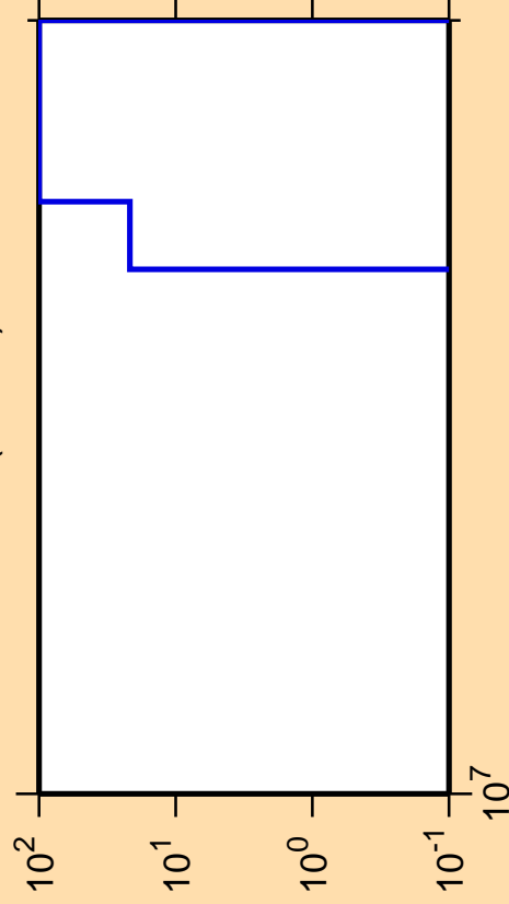
\Delta\sigma/\sigma vs. E for ^{177}\text{Ir} (mt 34)
