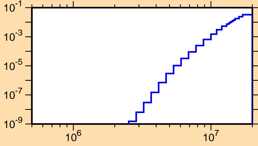
\sigma vs. E for ^{177}\text{Ir}(n,n\alpha)
