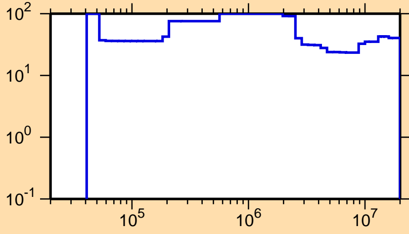
\Delta\sigma/\sigma vs. E for ^{177}\text{Ir}(n,\text{inel.})
