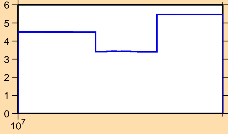
\Delta\sigma/\sigma vs. E for ^{177}\text{Ir}(n,\text{tot.})
