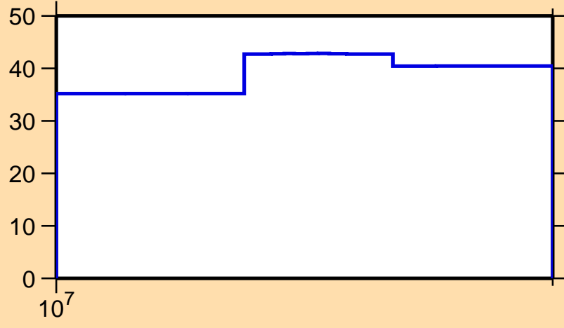
\Delta\sigma/\sigma vs. E for ^{177}\text{Ir}(n,\text{inel.})
