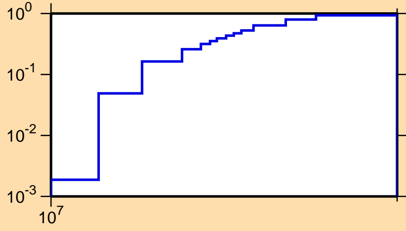
\sigma vs. E for ^{177}\text{Ir}(n,2n)
