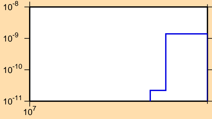
\sigma vs. E for ^{177}\text{Ir}(n,\text{pt})
