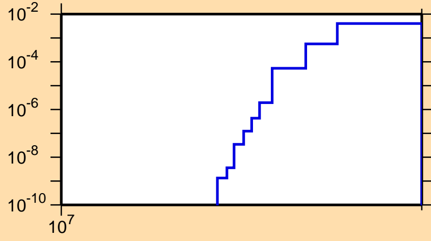
\sigma vs. E for ^{177}\text{Ir}(n,2np)
