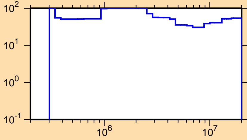
\Delta\sigma/\sigma vs. E for ^{177}\text{Ir}(n,n\text{cont.})
