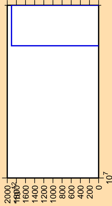
\Delta\sigma/\sigma vs. E for ^{177}\text{Ir} (mt 42)
