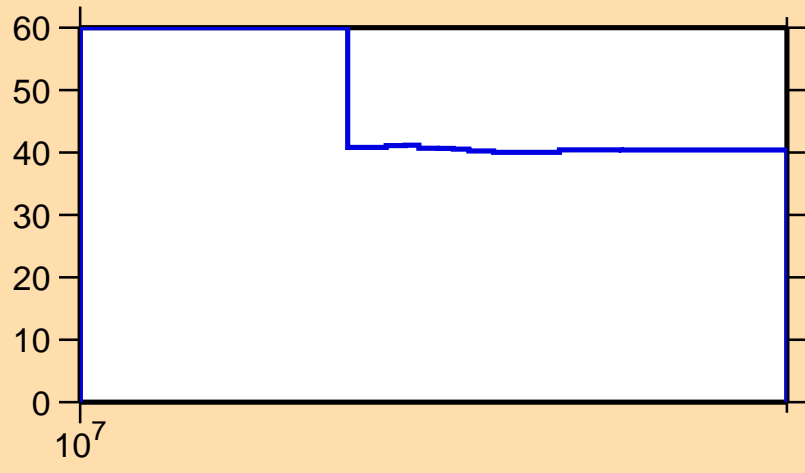
\Delta\sigma/\sigma vs. E for ^{177}\text{Ir}(n,2n)
