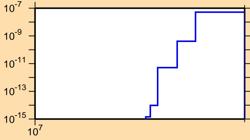
\sigma vs. E for ^{177}\text{Ir}(n,nt)
