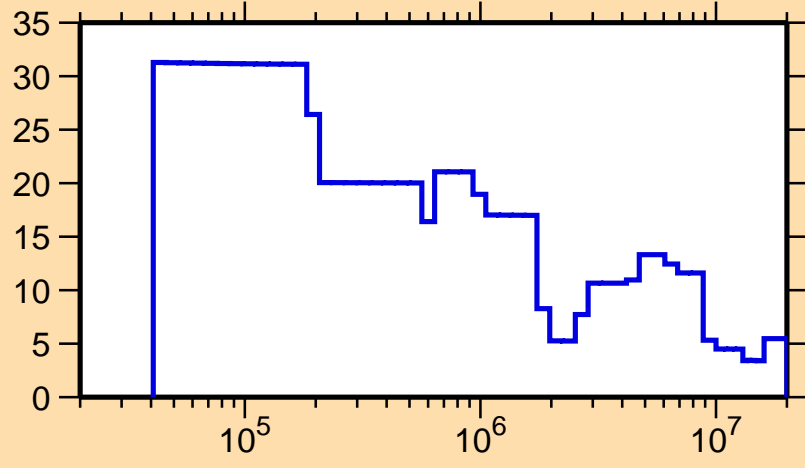
\Delta\sigma/\sigma vs. E for ^{177}\text{Ir}(n,\text{tot.})
