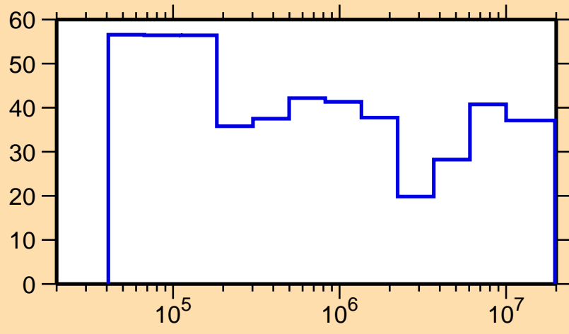
\Delta\sigma/\sigma vs. E for ^{177}\text{Ir}(n,n_1)
