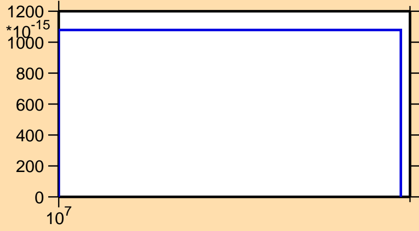
\sigma vs. E for ^{177}\text{Ir} (mt 34)
