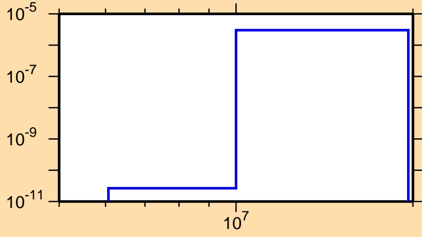
\sigma vs. E for ^{177}\text{Ir}(\text{mt } 45)
