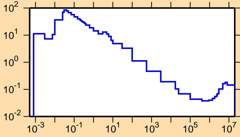
\sigma vs. E for ^{177}\text{Ir}(n,p)
