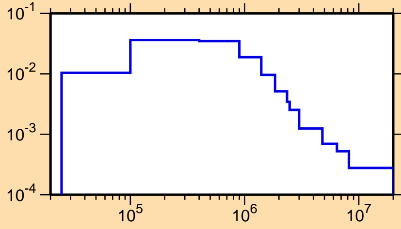
\sigma vs. E for ^{177}\text{Ir}(n,n_2)
