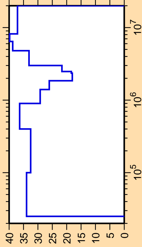
\Delta\sigma/\sigma vs. E for ^{177}\text{Ir}(n,n_2)
