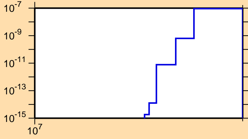
\sigma vs. E for ^{178}\text{Ir}(n,nt)
