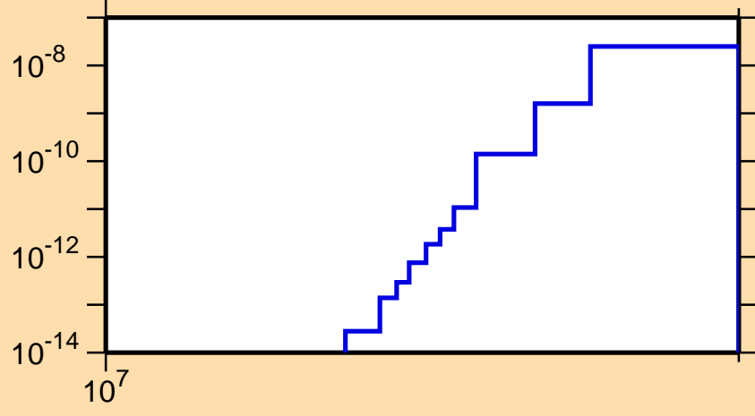
\sigma vs. E for ^{178}\text{Ir}(n,pt)
