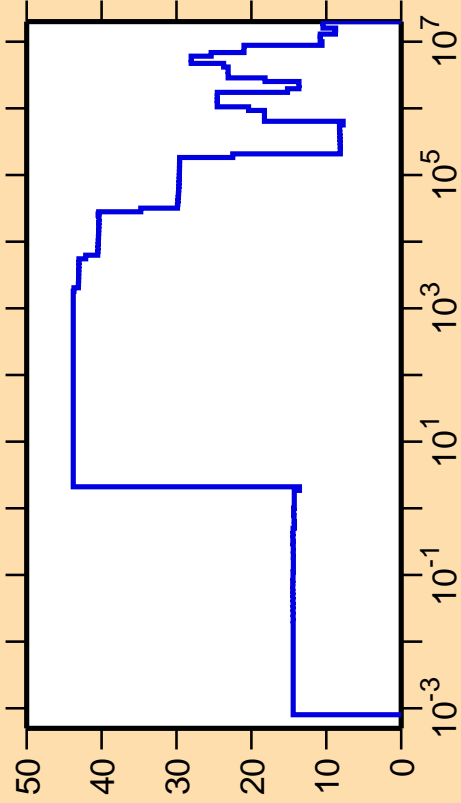
\Delta\sigma/\sigma vs. E for ^{178}\text{Ir}(n,\text{el.})
