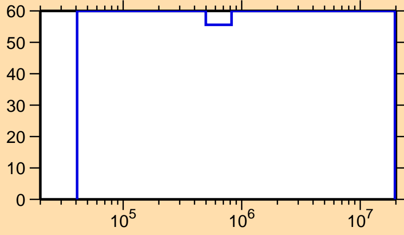
\Delta\sigma/\sigma vs. E for ^{178}\text{Ir}(n,n_1)
