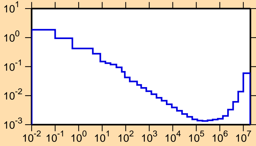
\sigma vs. E for ^{178}\text{Ir}(n,\alpha)
