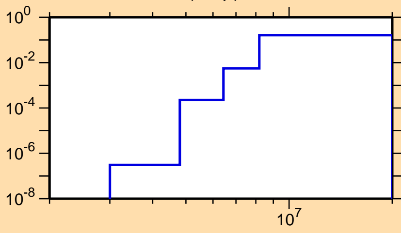
\sigma vs. E for ^{178}\text{Ir}(n,np)
