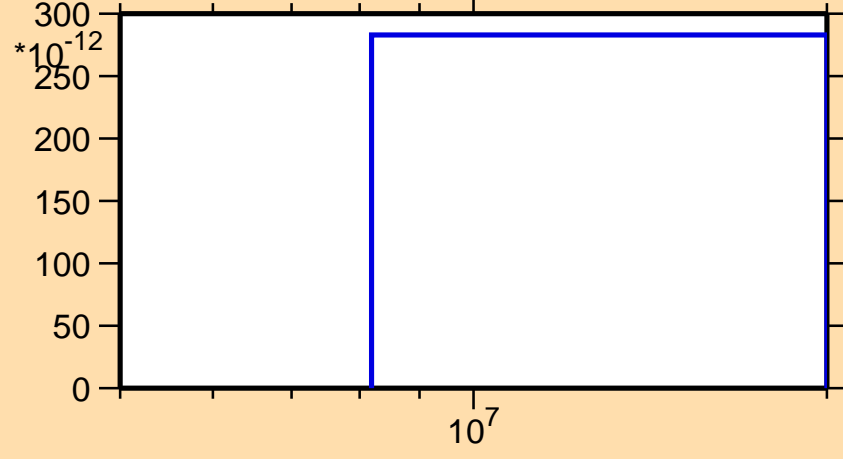
\sigma vs. E for ^{178}\text{Ir}(n,\text{pt})
