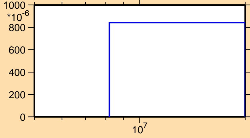
\sigma vs. E for ^{178}\text{Ir}(n,2np)
