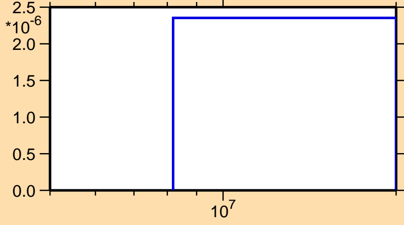
\sigma vs. E for ^{178}\text{Ir}(n,\text{nd})
