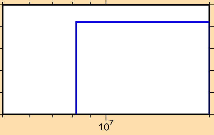
\sigma vs. E for ^{178}\text{Ir}(n,2np)
