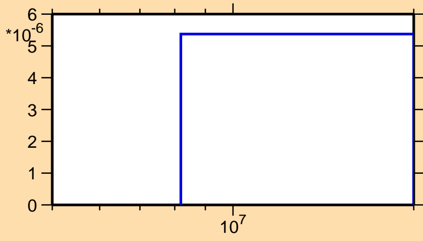
\sigma vs. E for ^{178}\text{Ir}(n,2n\alpha)
