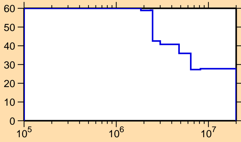
\Delta\sigma/\sigma vs. E for ^{178}\text{Ir}(n,n\text{cont.})
