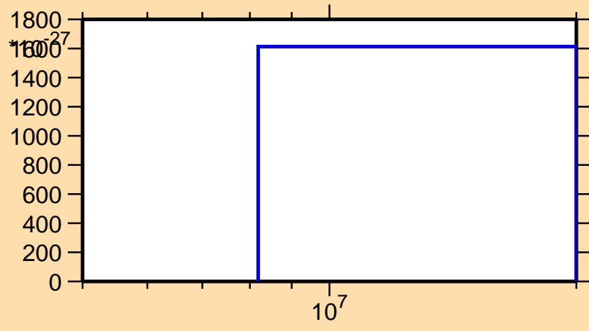
\sigma vs. E for ^{178}\text{Ir}(\text{mt } 42)
