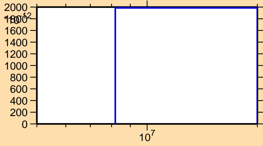
\sigma vs. E for ^{178}\text{Ir}(\text{mt117})
