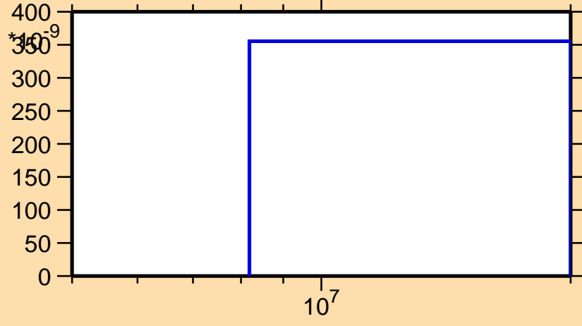
\sigma vs. E for ^{178}\text{Ir}(\text{mt } 45)
