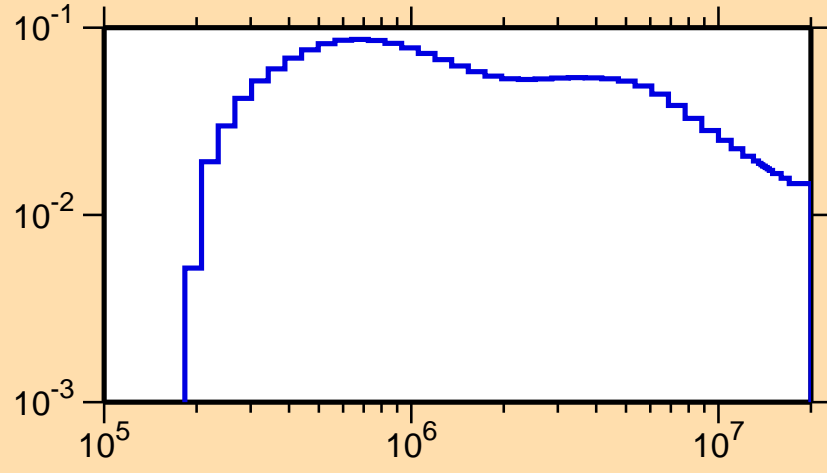
\sigma vs. E for ^{179}\text{Ir}(n,n_2)
