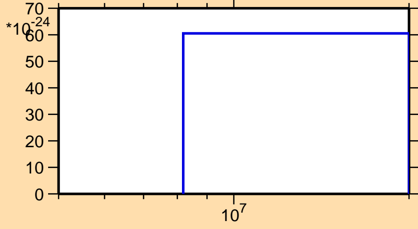
\sigma vs. E for ^{179}\text{Ir}(\text{mt } 42)
