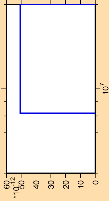
\Delta\sigma/\sigma vs. E for ^{179}\text{Ir}(\text{mt } 42)
