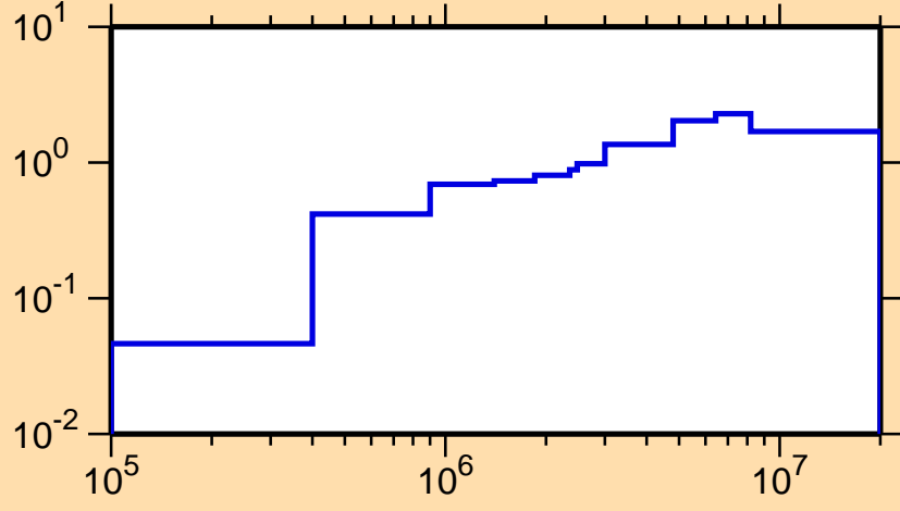
\sigma vs. E for ^{179}\text{Ir}(n,\text{inel.})
