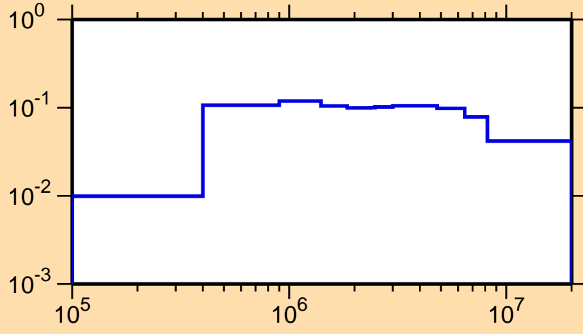
\sigma vs. E for ^{179}\text{Ir}(n,n_3)
