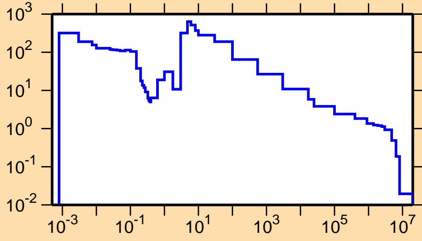
\sigma vs. E for ^{179}\text{Ir}(n,\gamma)
